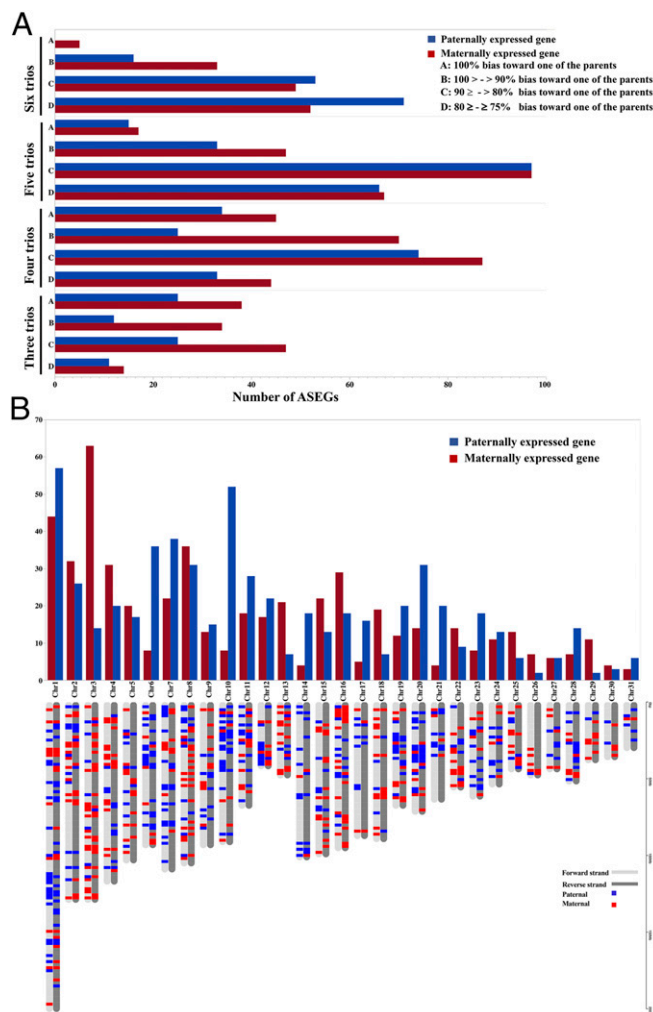
Fig. 2. (A) ASEGs in the individual parent–placenta trios. Combining the informative SNPs from all the trios may bias the results in identifying the ASEGs. Therefore, we analyzed the predicted ASEGs in each individual trio. The number of ASEGs in the parent–placenta trios are classified based on the number of trios that showed the informative SNPs. Red and blue bars indicate maternally and paternally expressed genes, respectively. (B) The distribution of ASEGs across equine chromosomes ( Top ). A total of 1,111 genes were located on autosomal chromosomes. ECA1 had the largest number of ASEGs among the autosomal chromosomes followed by ECA10, ECA3, and ECA7. A binomial test showed that there were biases in the proportion of maternal and paternal genes (toward one of the parents) in chromosomes on ECA3 and ECA10. ( Bottom ) Ideogram with the genomic map of the ASEGs. Distribution of paternally and maternally expressed genes are demonstrated based on the strand of their transcription. The ideogram was generated using Package “ChromoMap” in R (62). Gene names can be found in the interactive ideogram at https://rpubs.com/pouyadini/594229 .
