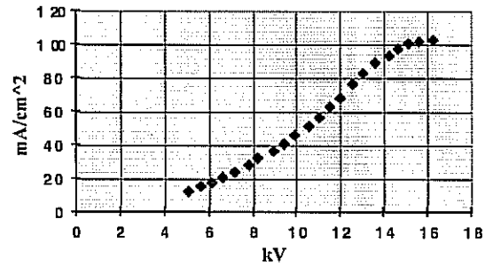
Figure 2: Current density versus extraction voltage.
