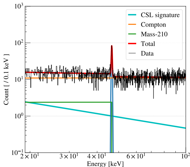
FIG. 1. The 95% CL spectral fit for the CSL radiation signature from wavefunction collapse. The 95% CL upper limit value for R_0 is 0.0368 /(\text{kg}\cdot\text{d}) .
