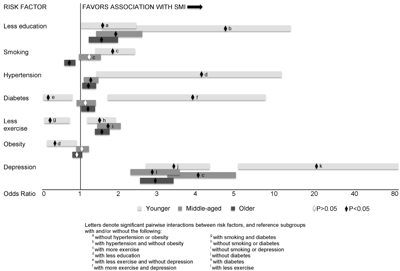
Figure 3. Odds Ratios and 95% Confidence Intervals for Subjective Memory Impairment (SMI) with each Risk Factor across Age Groups. doi:10.1371/journal.pone.0098630.g003
