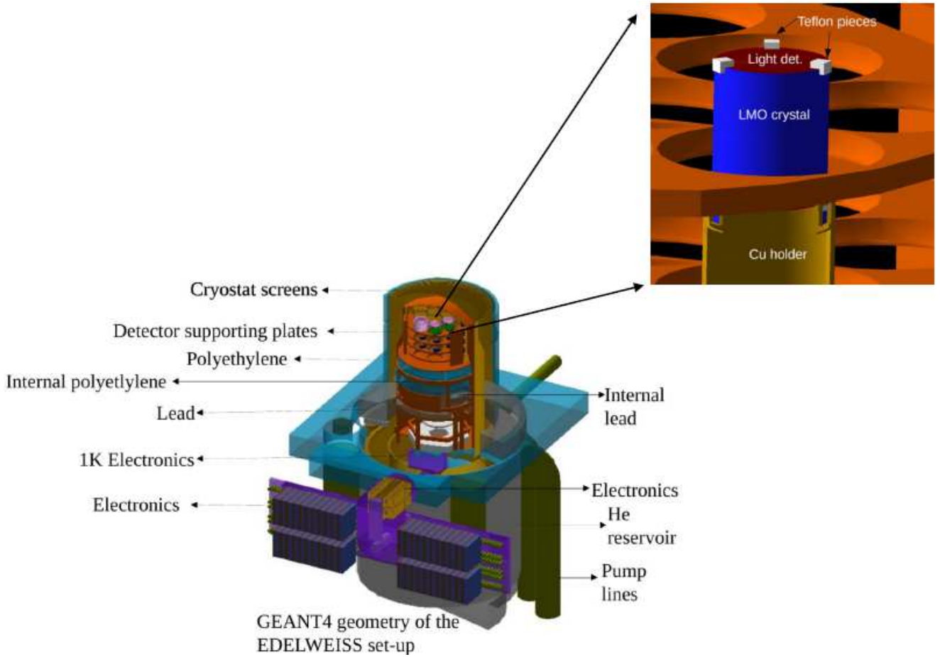
Fig. 1 EDELWEISS-III cryostat modeled in GEANT4 as configured for the experiment. (Zoom) The individual detectors are constructed from a crystal supported in a copper holder that also holds the light detector which is constructed with a Germanium wafer. The details of the copper assembly surrounding the crystals are not shown.
