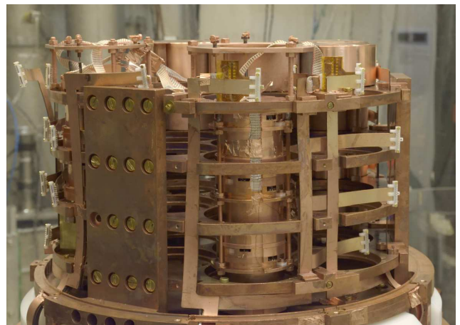
Fig. 2 EDELWEISS cryogenic facility with partially installed detector modules.
