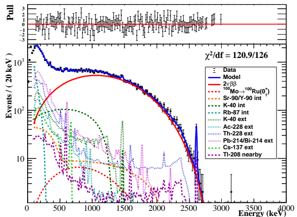
Fig. 4 Bottom: The energy spectrum accumulated with \text{Li}_2^{100}\text{MoO}_4 scintillating bolometers (exposure is 42.235 \text{ kg}\times\text{d} ) and the fit in the energy range [120 – 3000] keV. The data points represent the data, the solid blue line shows the sum of all components of the fit, the solid red line is the 2\nu\beta\beta contributions, and the other components of the fit are described in the legend. Top: fit residuals normalized by the statistical error of the data in each energy bin (“pulls”).
