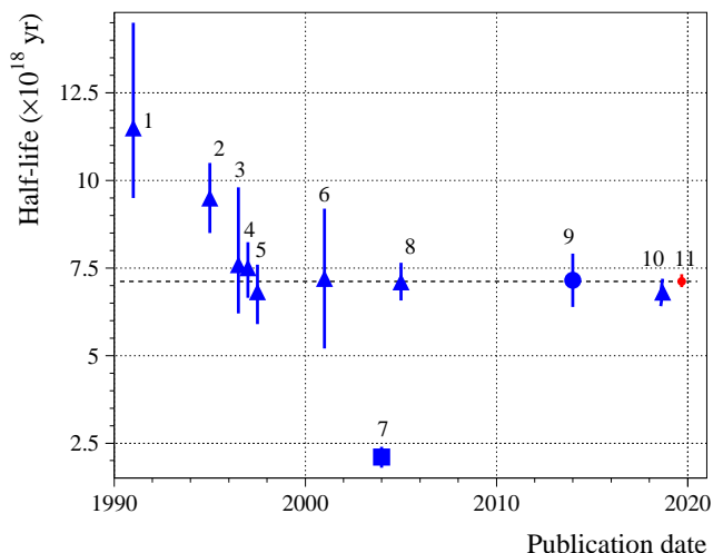
Fig. 6 A historical perspective of T_{1/2}^{2\nu} of ^{100}\text{Mo} as a function of the publication date in the experiments: (1) ELEGANT V [5], (2) NEMO-2 [6], (3) segmented Si(Li) detector [8], (4) NEMO-2 reanalyzed [7], (5) Hoover Dam using a time-projection chamber [9], (6) DBA (liquid argon detector) [10], (7) geochemical experiment [11], (8) preliminary result of NEMO-3 [12], (9) low temperature \text{ZnMoO}_4 bolometers [13], (10) final result of NEMO-3 [14], (11) present study.
