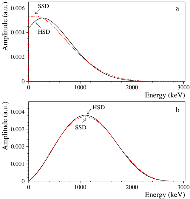
Fig. 5 Single-electron spectra (a) and summed energy spectra of two electrons (b) for the ^{100}\text{Mo} \rightarrow ^{100}\text{Ru} 2\nu\beta\beta decay calculated in the HSD and SSD models. The spectra are normalized to unit area.
