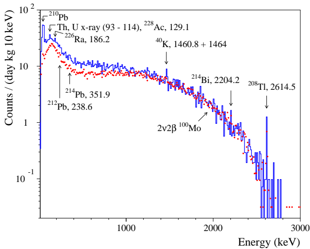
Fig. 3 Energy spectra accumulated with the \text{Li}_2^{100}\text{MoO}_4 scintillating bolometers in the setup 1 (solid blue histogram, exposure 10.308 kg \times d) and setup 2 (red dotted histogram, exposure 31.927 kg \times d). The \gamma -ray energies are listed in keV.
