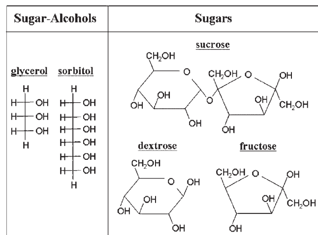
Fig. 1. Chemical structure representations of sugar-alcohols and sugars.
