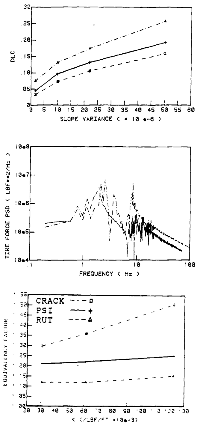
Fig.9 Effect of Spring Stiffness on Vehicle Response and Road Damage a) Leading Drive Axle DLC versus SV \square - - - K = 30,600 lbs/ft + - - - K = 61,200 lbs/ft ( standard ) \triangle - - - K = 122,400 lbs/ft b) Leading Drive Axle Tire Force PSD at SV = 22 \times 10^{-6} c) Effect of Leaf Spring Stiffness on Pavement Damage
