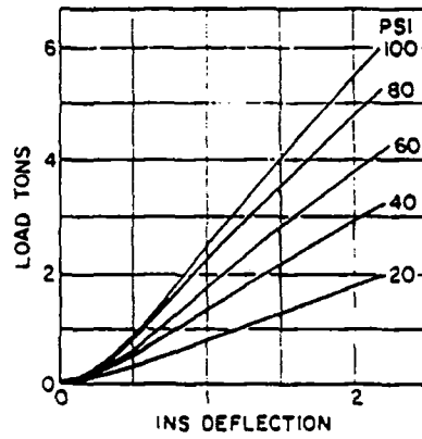
11.00 x 20 tire deflection data over a range of pressures.
