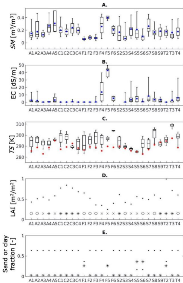
Fig. 2. Boxplots showing the within-pixel variability of in situ measurements for the visited EASEv2 pixels, for A. soil moisture ( SM ), B. salinity ( EC ) and C. soil temperature ( T_5 ). The blue and red dots indicate the upscaled EASEv2 pixel value, with the red dots representing soil temperature extrapolated to 6 am. Also shown are D. July-August 2019 average of MODIS-derived LAI (.) and in situ observed vegetation class, with o = mixed forest, * = agriculture and x = open shrubland, and E. HWSD-derived sand (.) and clay (*) fraction. Sampling dates differ across pixels and range from July 19 to August 27, 2019 (Table I).
