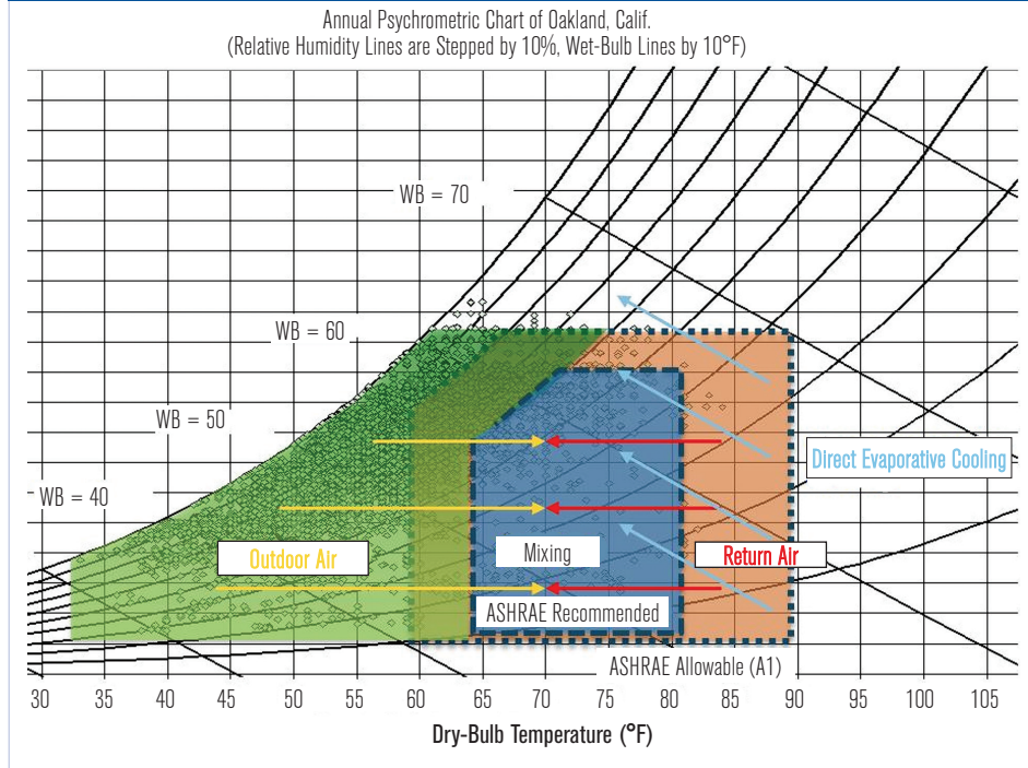
FIGURE 3 Psychrometric chart showing Oakland weather and cooling strategies.
