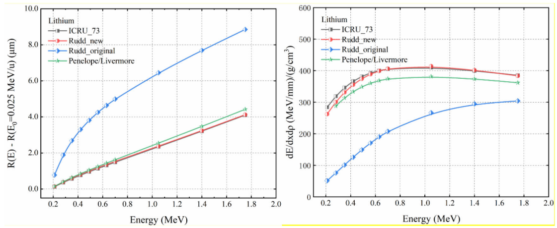
Figure 3. Range and stopping power of Lithium in the liquid water calculated with different cross-sections or physics models
