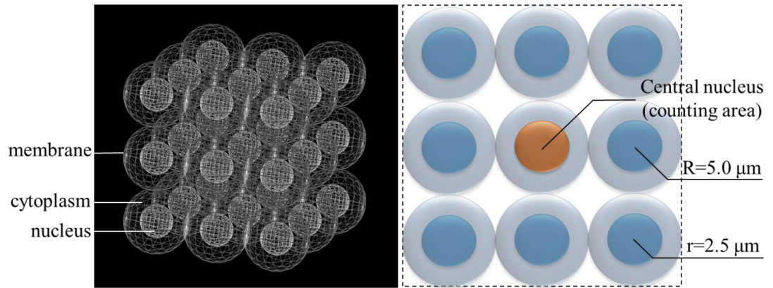
Figure 1. Geometric model for lineal energy calculation shown in Qt5 and its sectional view
