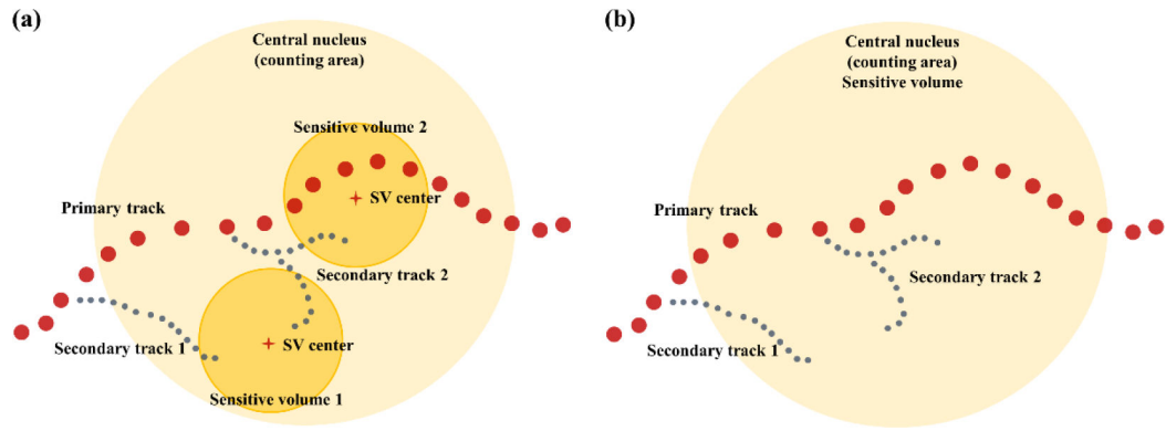
Figure 2. Schematic of lineal energy calculation: (a) nano-SV (radius = 1 nm) (b) micron-SV (radius = 2.5 μm). The volumes of SVs and nuclei are for visual display and do not represent the actual size.
