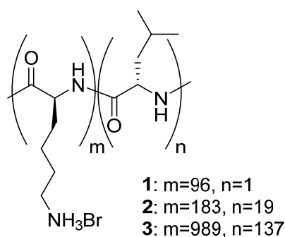
Figure 1. Chemical structures of the diblock copolypeptide amphiphiles \text{K}_{96}\text{L}_1 ( 1 ), \text{K}_{183}\text{L}_{19} ( 2 ) and \text{K}_{989}\text{L}_{137} ( 3 ).
