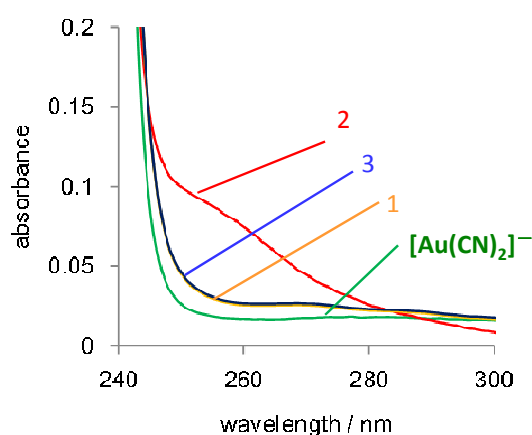
Figure 2. UV-vis absorption spectra of composites 1 / [Au(CN)_2]^- , 2 / [Au(CN)_2]^- and 3 / [Au(CN)_2]^- in deionized (DI) water. [Au(CN)_2]^- = 0.2 mM (Lys units: K[Au(CN)_2] = 1:1 ).
