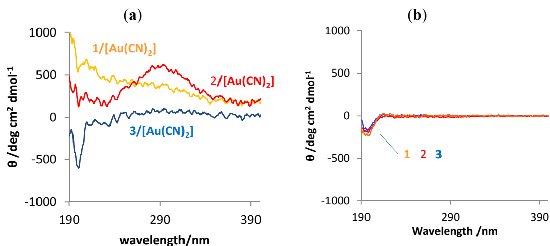
Figure 3. (a) Circular dichroism (CD) spectra of 1 /[Au(CN) 2 ] − , 2 /[Au(CN) 2 ] − and 3 /[Au(CN) 2 ] − in DI water. [Au(CN) 2 ] − = 0.2 mM. (Lys units:K[Au(CN) 2 ] = 1:1). (b) CD spectra of 1 , 2 and 3 in DI water ([Lys unit] = 0.2 mM).
