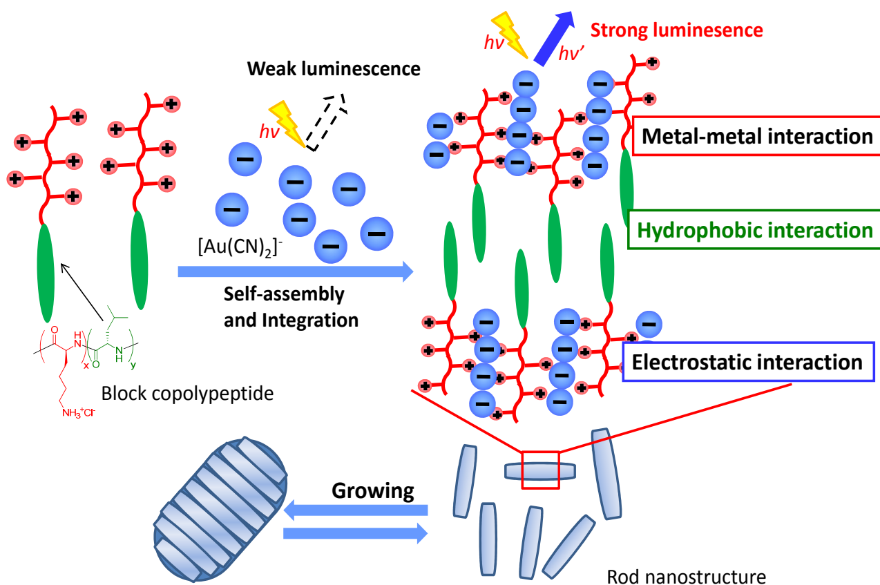
Figure 8. Schematic illustration of self-assembly of copolypeptide amphiphiles/Au complexes to develop the functional nanostructure.
