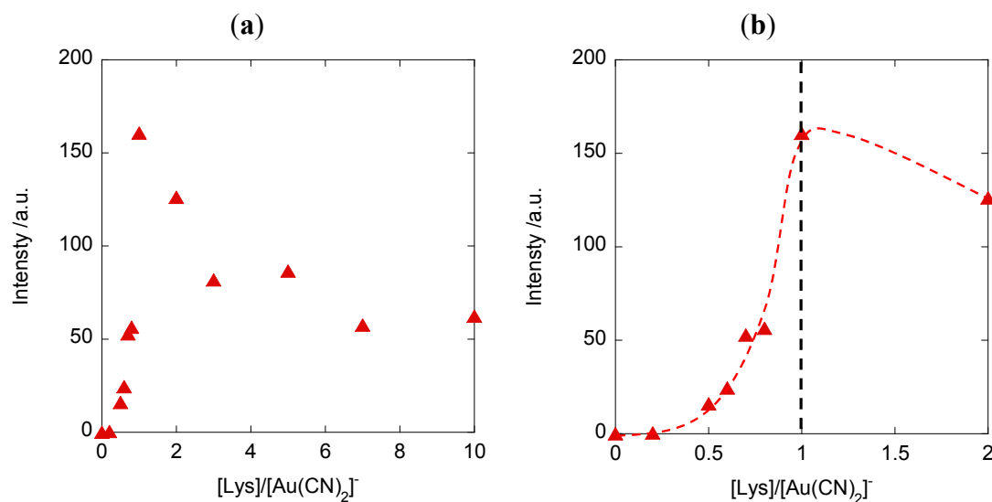
Figure 5. (a,b) Variations in the fluorescent intensity of 2 / [\text{Au}(\text{CN})_2]^- with changes in the lysine: [\text{Au}(\text{CN})_2]^- molar ratio (a: 0–10, b: 0–2) in DI water. (c) Variations in the fluorescence wavelength of 2 / [\text{Au}(\text{CN})_2]^- with changes in the lysine: [\text{Au}(\text{CN})_2]^- molar ratio in DI water. [\text{Au}(\text{CN})_2]^- = 0.2 \text{ mM} .
