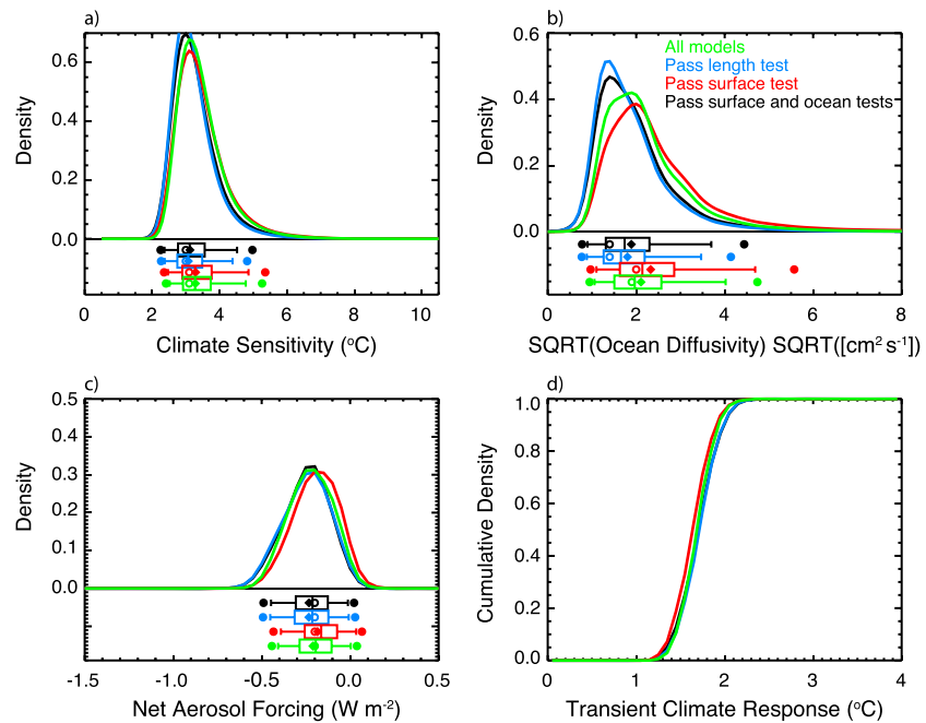
Figure 3. Marginal probability distribution functions for effective climate sensitivity (a), \sqrt{K_v} (b), and F_{aer} (c) and cumulative distribution function for transient climate response (d) resulting from merging the variability estimates across models with similar characteristics. Groupings are for all models (green), all models with length greater than 500 years (blue), all models with median parameters consistent with global mean temperature change (red), and all models with median parameters consistent with global mean temperature change and ocean heat content change (black). Colors for the merged groups are chosen so that the color of the last test passed before failure matches that from Figure 1 (e.g., models that fail all tests are plotted green in Figure 1 and therefore only fit in the “all models” group).
