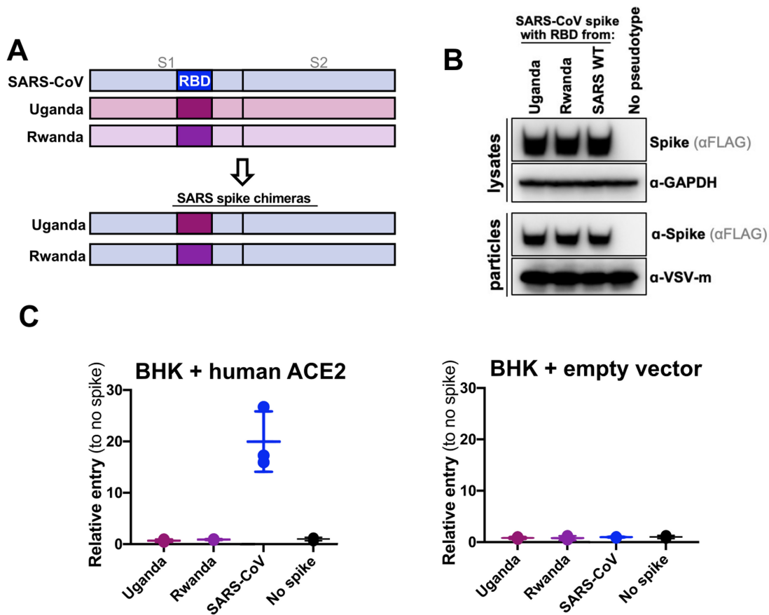
Figure 3. hACE2 usage of bat sarbecoviruses investigated using a surrogate VSV-pseudotyping system. (A) Schematic showing the structure of chimeric spike proteins. The SARS-CoV-1 spike backbone is used in conjunction with the RBD from the Uganda and Rwanda strains. (B) Incorporation of chimeric SARS-CoV-1 spike proteins into VSV. Western blots show successful expression of chimeric spikes (lysates) and their incorporation into VSV (particles). (C) hACE2 entry assays. Left, wildtype SARS-CoV spike protein is able to mediate entry into BHK cells expressing hACE2. In contrast, recombinant spike proteins containing either the Uganda or Rwanda RBD were unable to mediate entry. Entry is expressed relative to VSV particles with no spike protein. Right, control experiment for entry assay. BHK cells do not express hACE2 and therefore do not permit entry of hACE2-dependent VSV pseudotypes.
