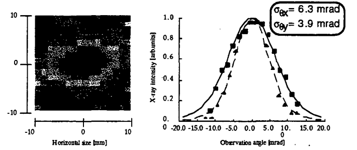
Figure 3. a) False color CCD image of the spatial profile of a 30 keV x-ray pulse on the phosphor screen, which is located 80 cm from the IP; b) \blacksquare (square)- horizontal line-profile and fitting curve (solid line), \blacktriangle (triangle) -vertical line-profile and fitting curve (dashed line) from Fig. 3 (a). The scale has been converted into angular units.
