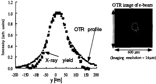
Figure 2: a) OTR image of the focused electron beam and b) \blacktriangle (triangle) - vertical line-profile through the OTR image of the electron beam; \blacksquare (square)- x-ray yield vs. vertical laser beam position.
