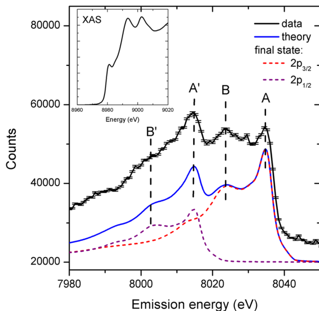
FIG. 2. HEROS spectra of Cu metal for 2000 self-seeded shots (black curve). The error bars represent the standard deviation of the total counts. For comparison, we plot the calculated spectrum using the Kramers-Heisenberg relation and a Cu K-edge XAS spectrum recorded at a synchrotron facility shown in inset. The calculated curve represents the sum of two spectra relating to the final electronic states of 2p_{3/2} and 2p_{1/2} . Reproduced with the permission from Struct. Dyn. 1 , 021101 (2014). Copyright 2014 AIP Publishing LLC.
