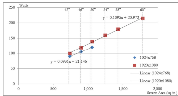
Figure 4-18. On-Mode Power of Panasonic PDP TVs
