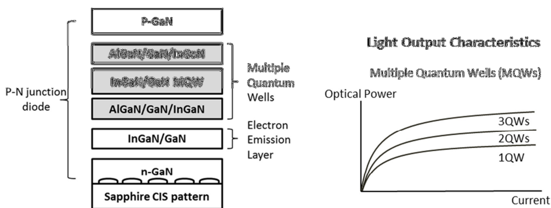
Figure 4-7. Example of LED Structure with Multiple Quantum Wells (MQWs)
