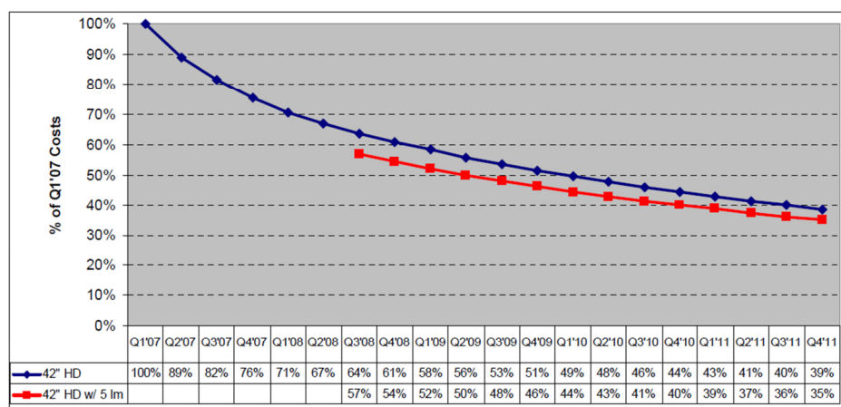
Figure 4-21. Indexed 42-inch HD Plasma Panel Costs at 2.5 lm/W and 5.0 lm/W
