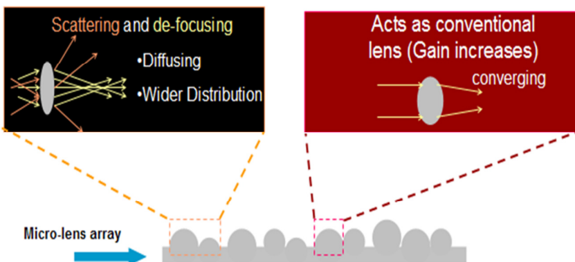
Figure 4-12. Mechanism of Micro-lens Films
