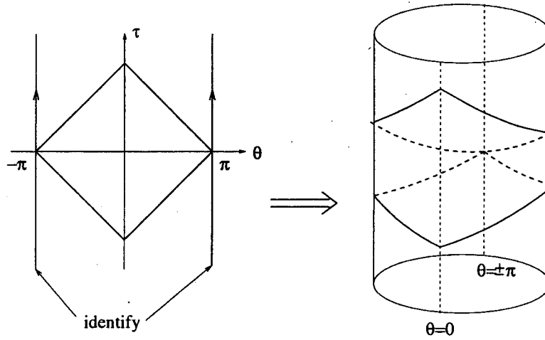
Figure 2.2: The rectangular region can be embedded in a cylinder, with \theta = \pi and \theta = -\pi being identified.
