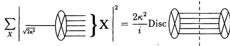
Figure 1.3: An application of the optical theorem.
