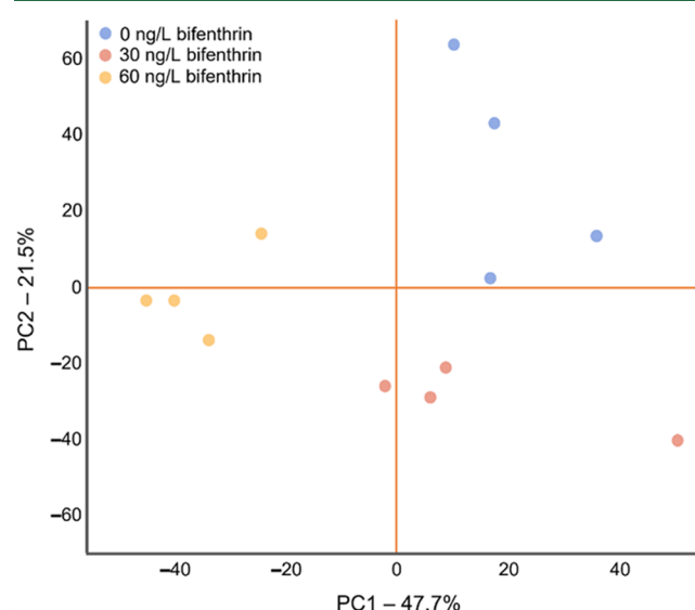
Figure 1. Principle component analysis (PCA) of the total lipid content in juvenile rainbow trout exposed to 0, 30, and 60 ng/L bifenthrin ( n = 4 per treatment).
