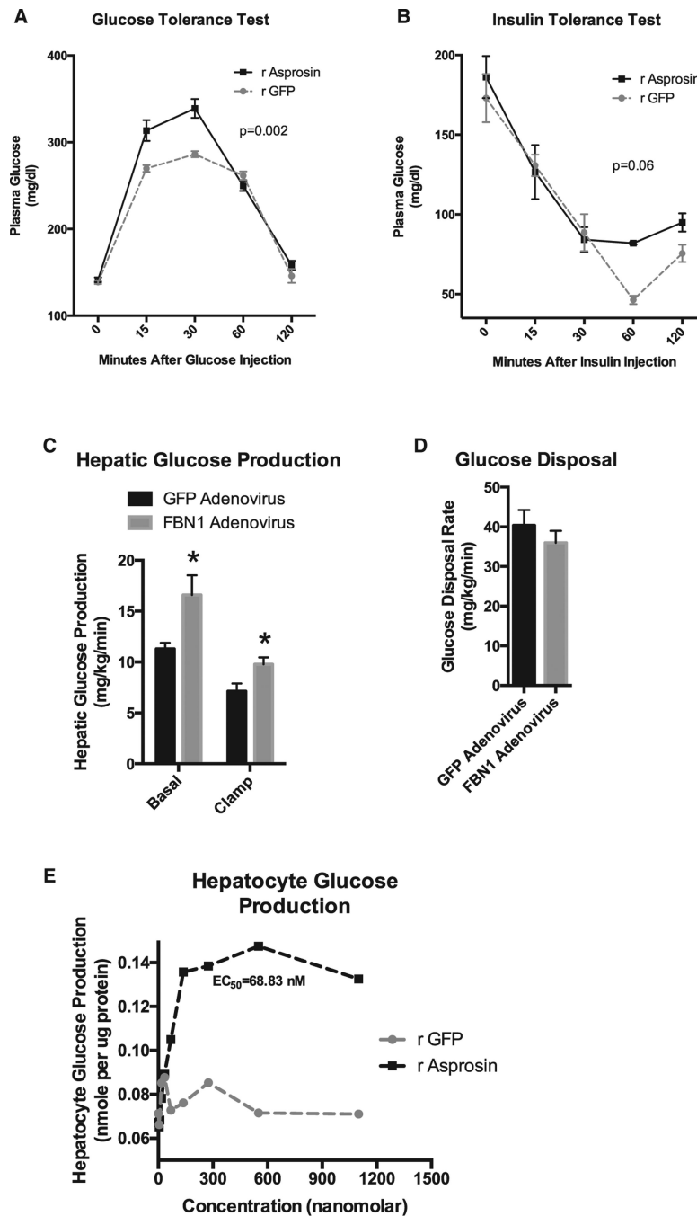
Figure 4. In a Cell-Autonomous Effect, Asprosin Targets the Liver to Increase Plasma Glucose (A) A glucose tolerance test was performed 2 hr following a subcutaneous injection with 30 mg recombinant asprosin or GFP in WT mice fasted for 2 hr for synchronization prior to injection (n = 6 mice in each group). Two-way ANOVA with Bonferroni post test was used to calculate the p value. (B) An insulin tolerance test was performed 2 hr following subcutaneous injection with 30 \mu g recombinant asprosin or GFP in WT mice fasted for 2 hr for synchronization prior to
