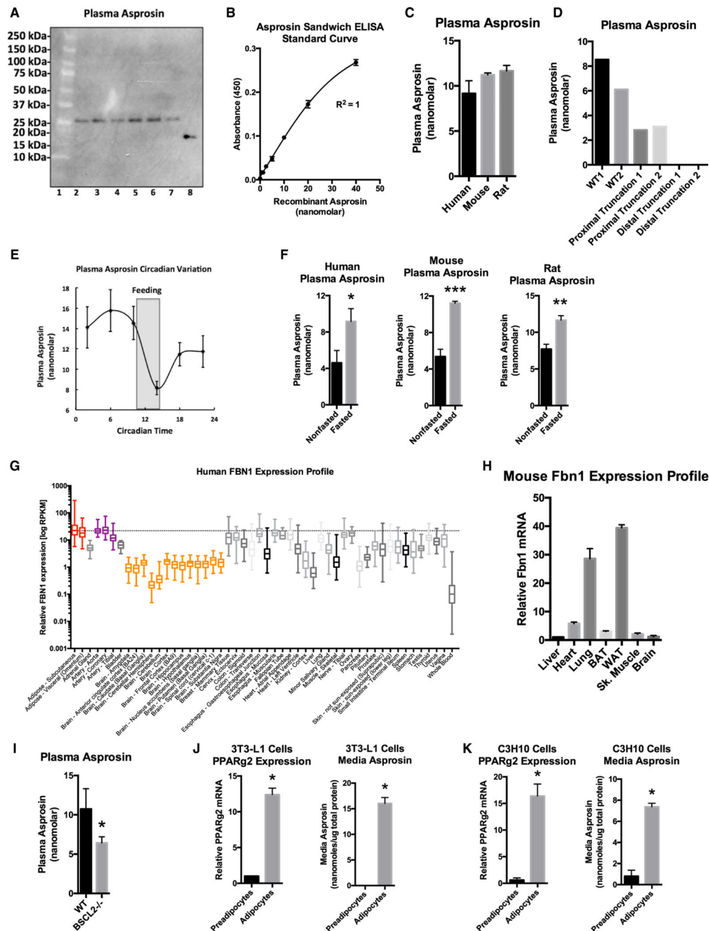
Figure 2. Asprosin, the C-Terminal Cleavage Product of Profibrillin, Is a Fasting-Responsive Plasma Protein
