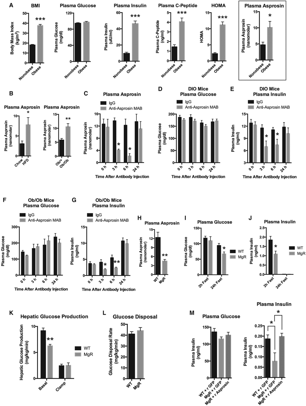
Figure 7. Immunologic or Genetic Asprosin Loss of Function Reduces Hepatic Glucose Production, Plasma Glucose, and Plasma Insulin
