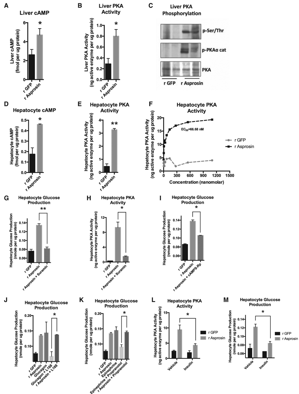
Figure 6. Asprosin Uses the cAMP Second-Messenger System and Activates PKA in the Liver
