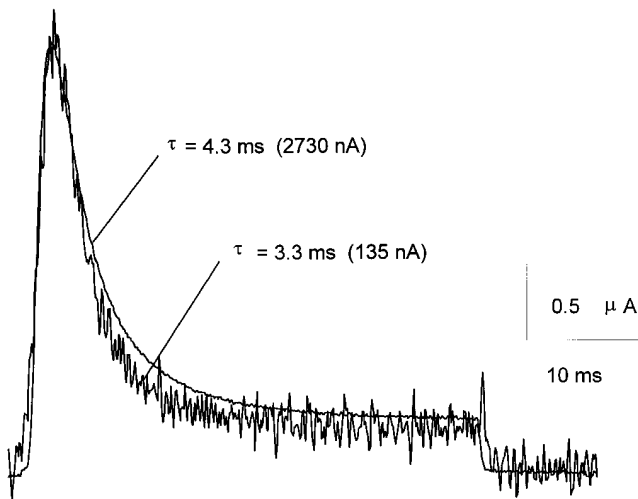
FIGURE 9. ShH4 ionic current evoked by a 40-ms depolarizing pulse to 20 mV, just before and after 24 min of internal perfusion of an oocyte with NMDG-Glu ( 400 \mu\text{l/h} ). The traces are scaled to the peak current, with amplitudes indicated next to the corresponding trace. In this cell, ionic current decayed with a time constant of 4.3 ms at the beginning of the experiment, and of 3.3 ms 24 min later, as the peak current was only 5% of the initial one. The perfusion pipette was placed close to the cytoplasmic face of the dome membrane. The current was monitored every 5 s, from a HP = -90 mV. The top and guard solution was NaMES Ca2, the bottom and perfusion pipette solution was NMDG-Glu. The data were sampled at 10 kHz and filtered at 2 kHz. A P/ -4 protocol from SHP = -90 mV was used for leak subtraction.
