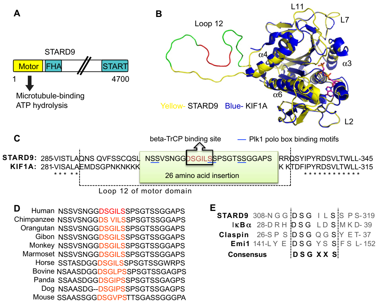
FIGURE 1: The STARD9 motor domain loop 12 harbors a unique insertion with Plk1 and \beta -TrCP binding sites. (A) Schematic of the STARD9 modular domain composition. (B) Molecular modeling of the STARD9 motor domain using the KIF1A motor domain crystal structure (PDB ID 11A0). Note that loops 7, 11, and 12 are extended. (C) Compared with KIF1A, STARD9 contains a 26-amino acid insertion in loop 12 with putative Plk1 polo-box domain-binding motifs (SS) and a \beta -TrCP DSGXXS-binding motif. (D) The 26-amino acid insertion and DSGXXS motif are highly conserved among STARD9 mammalian orthologues. (E) Alignment of STARD9, I \kappa B \alpha , claspin, and Emi1 \beta -TrCP DSGXXS-binding motifs and consensus.
