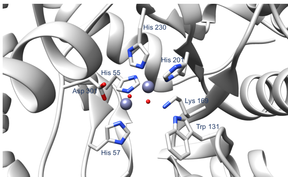
Figure 2. The OPH active site, highlighting the amino acid residues that coordinate the two Zn(II). Other important residues involved in the catalytic activity of the enzyme are Trp 131 and Lys 169. The PDB used to produce this figure is 1HZY. The Zn(II) ions and the water molecules are shown in purple and red spheres, respectively.
