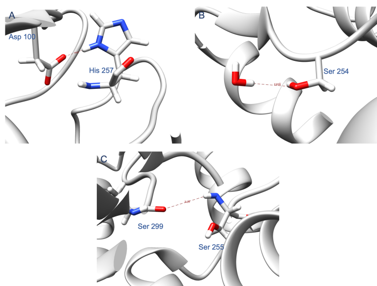
Figure A6. Hydrogen bonds formed during MD simulations on OPH mutants. (A) The hydrogen bond found during MD simulation on the double mutant D253E-I255G complexed to paraoxon between Asp 100 and His 257. (B) The hydrogen bond found during MD simulation on OPH:H254S between a crystal water molecule and the mutated residue H254S. (C) The hydrogen bond found during MD simulation on OPH:I255S between the mutated residue I255S and Ser 299.
