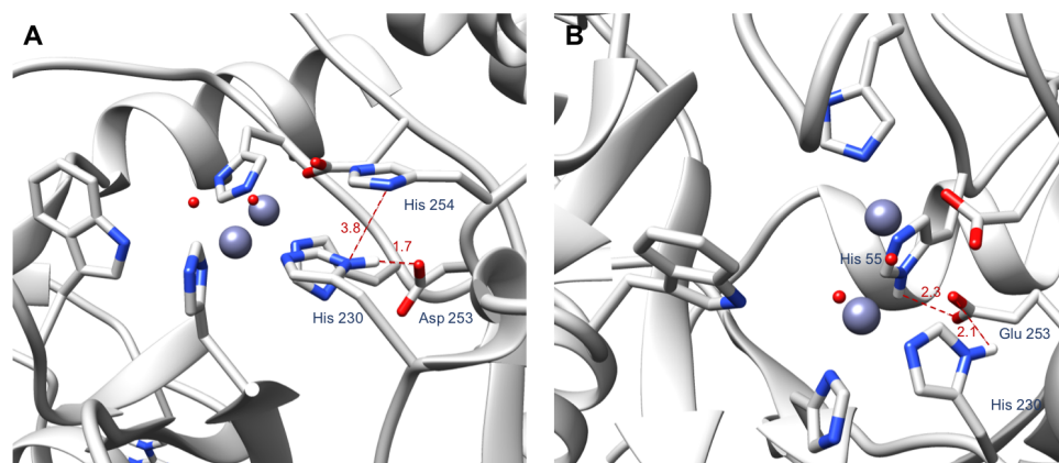
Figure 5. The binding site of OPH. (A) Figure showing the hydrogen bond between His 230 and Asp 253 and the stacking between His 230 and His 254. (B) Figure showing the hydrogen bonds that Glu 253 establishes with His 55 and His 230. The Zn(II) ions and the water molecules are represented in purple and red spheres, respectively. Only the hydrogen atoms involved in the highlighted interactions are shown.
