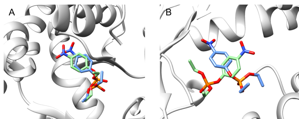
Figure 4. Superimposition of the docking poses before (in green) and after (in blue) MD simulations within the OPH catalytic site. To evaluate the stability of our docking poses during MD simulations, we calculated the RMSD of each pose at the end of the MD trajectories (15 ns) relative to the starting pose. Here, we report in: (A) the most stable binding pose with the lowest RMSD value of 1.77 Å; this pose was generated using HYBRID, and (B) the docking pose that reproduces the binding mode of the substrate analog; it was generated using POSIT (OEDocking 3.2.0; OpeneEye Inc.). Contrary to our expectations, we found that this binding mode is not stable (RMSD of 6.6 Å), highlighting that the binding mode of the substrate analog does not reflect the binding mode of paraoxon.
