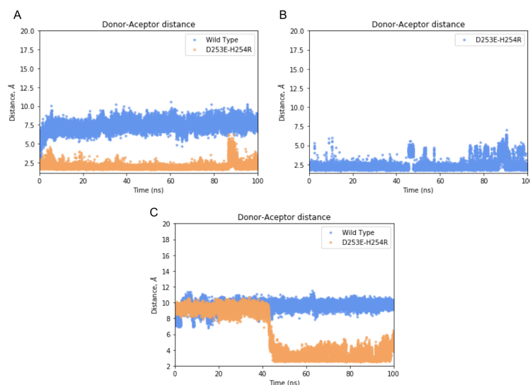
Figure A3. The donor-acceptor distances found during 100 ns of MD simulation on WT OPH complexed to paraoxon and the double mutant D253E-H254R complexed to paraoxon between: (A) The residue at position 254 (His in WT OPH and Arg in the double mutant) and Leu 271, (B) Arg 254 and His 257, and (C) Asp 100 and Lys 169. We found that during the simulations on the double mutant (D253E-H254R) complex, the distances between: (i) H/R 254 and Leu 271, (ii) Arg 254 and His 257, and (iii) Asp 100 and Lys 169 are short (fluctuating around 2 Å), signaling the formation of hydrogen bonds between the residues belonging to each of these pairs. The respective donor-acceptor distances during MD simulation on the WT OPH complex are greater than the typical distance of a hydrogen bond (2 Å). The distance between residues Arg 254 and His 257 corresponding to the WT complex are not shown on the plots of this figure since Arg 254 was found far from the residue at position 257 during the respective MD simulations. These results show that the double mutant D253E-H254R induced three different hydrogen bonds near the active site of OPH. Pictorial representations of these interactions are shown on Figure A4.
