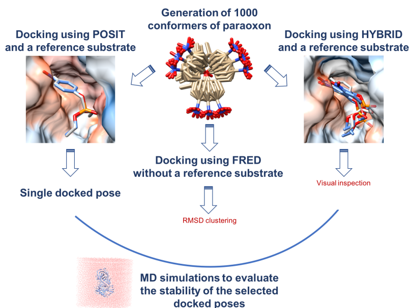
Figure 3. A schematic description of our docking protocol involving three different docking tools (POSIT, HYBRID, and FRED) from OpenEye Toolkits used to dock paraoxon in the active site of OPH.
