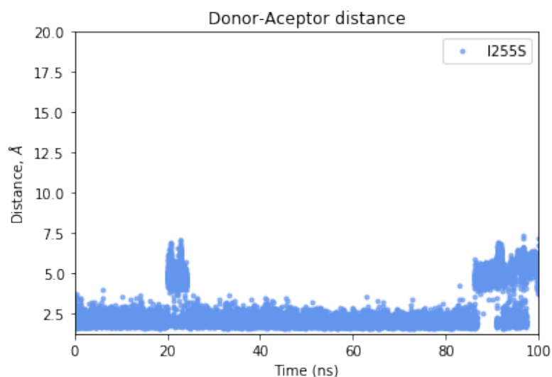
Figure A8. The donor-acceptor distance found during 100 ns of MD simulation on OPH:I255S between the mutated residue I255S and Ser 299. These two residues establish a stable hydrogen bond with a distance fluctuating around 2 Å. A pictorial representation of this interaction is shown on Figure A6C.
