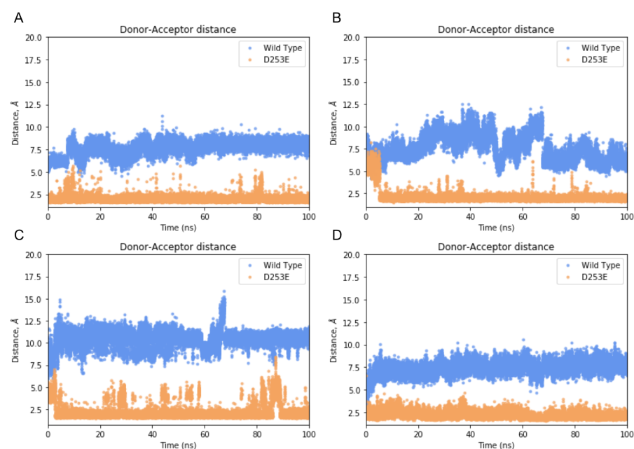
Figure A1. The donor-acceptor distances found during 100 ns of MD simulation in Wild Type OPH complexed to paraoxon and the mutant D253E complexed to paraoxon between: (A) Thr 54 and His 55, (B) His 57 and Trp 302, (C) Thr 200 and His 201, and (D) Leu 271 and His 254. We found that, during the simulations on the OPH variant (D253E) complex, the distances between: (i) Thr 54 and His 55, (ii) His 57 and Trp 302, (iii) Thr 200 and His 201, and Leu 271 and His 254 are short (fluctuating around 2 Å), signaling the formation of hydrogen bonds between the residues belonging to each of these pairs. The respective donor-acceptor distances during MD simulation on the WT complex are greater than the typical distance of a hydrogen bond (2 Å). These results show that the mutation D253E induced four different hydrogen bonds near the active site of OPH. Pictorial representations of these interactions are shown on Figure A2.
