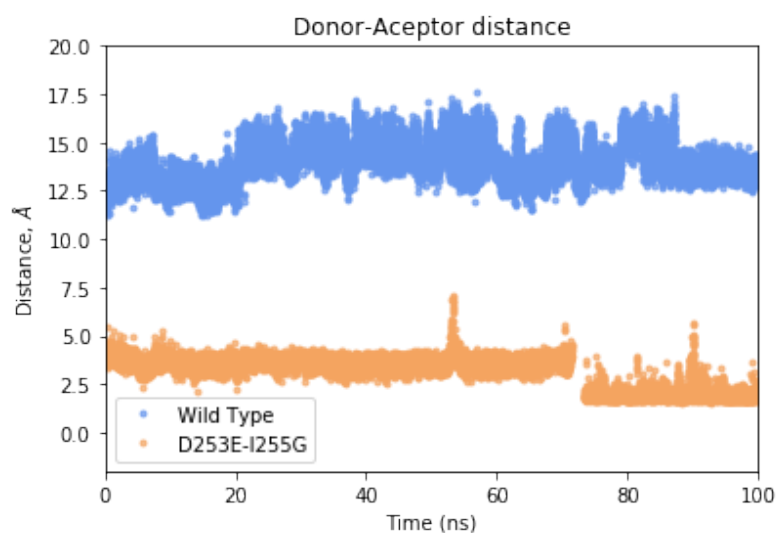
Figure A5. The donor-acceptor distances found during 100 ns of MD simulation on WT OPH:paraoxon complex and the double mutant D253E-I255G complexed to paraoxon between Asp 100 and His 257. These residues do not interact during the simulations of the WT complex. Asp 100 and His 257 are closer during the simulations of the double mutant complex compared to the simulations on the WT complex. In addition, these residues come close after 75 ns of MD on the mutant complex (D253E-I255G), where they establish a stable hydrogen bond with a distance fluctuating around 2 Å. This close contact is lost around 75 ns due to a wide opening of the protein's structure which resulted in a distance between Asp 100 and His 257 higher than 20 Å, leading to missing data points around 75 ns. A pictorial representation of this interaction is shown on Figure A6A.
