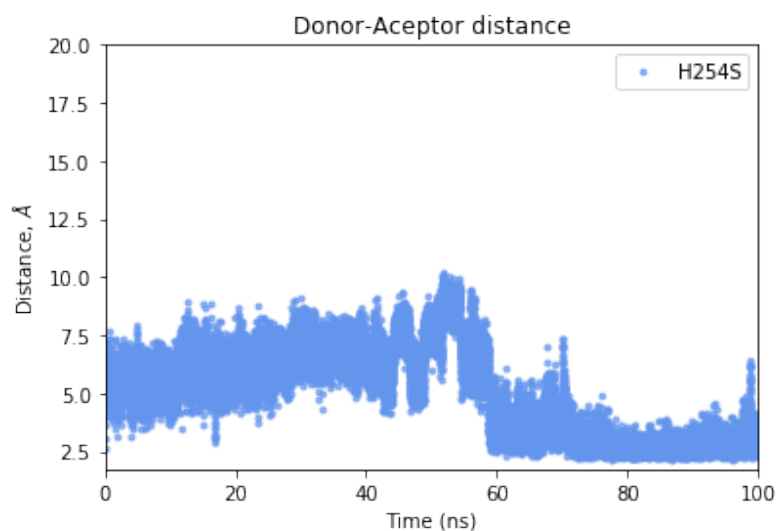
Figure A7. The donor-acceptor distance found during 100 ns of MD simulation on OPH:H254S between a crystal water molecule and the mutated residue H254S. After 60 ns of MD on the mutant complex (H254S), a water molecule belonging to the active site of OPH and involved in the coordination of Zn(II) establishes a hydrogen bond with Ser 254 with a distance fluctuating around 2.5 Å. A pictorial representation of this interactions is shown on Figure A6B.
