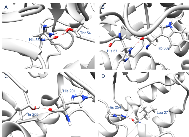
Figure A2. The donor-acceptor distances found during MD simulation of the mutant D253E complexed to paraoxon between: (A) Thr 54 and His 55, (B) His 57 and Trp 302, (C) Thr 200 and His 201, and (D) Leu 271 and His 254. These results show that the mutation D253E induced four different hydrogen bonds near the active site of OPH.
