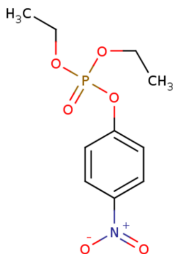
Figure 1. Representation of the 2D structure of paraoxon, which was generated using the ChemDB Chemoinformatics Portal ( http://chemdb.ics.uci.edu ), accessed on 11 November 2021.
