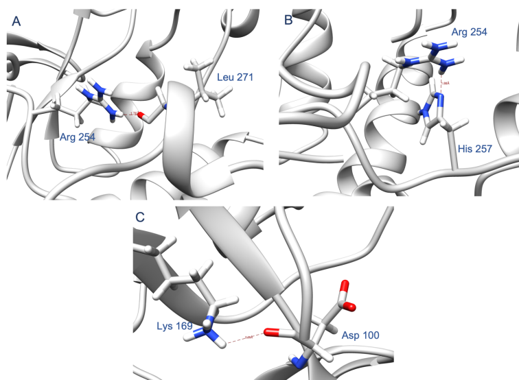
Figure A4. The donor-acceptor distances found during MD simulation on the double mutant D253E-H254R complexed to paraoxon between: (A) Arg 254 and Leu 271, (B) Arg 254 and His 257, and (C) Asp 100 and Lys 169. These results show that the double mutant D253E-H254R induced three different hydrogen bonds near the active site of OPH.
