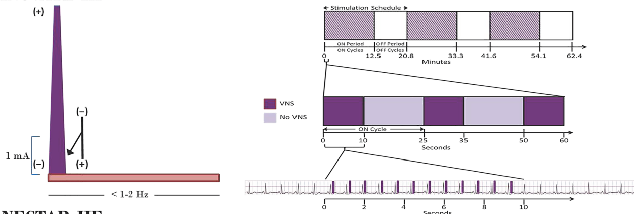
Figure 4 Differences in vagal nerve stimulation polarity, pulse frequency, and stimulation schedules across studies. A very complex repetitive schedule of stimulation was utilized in increase of vagal tone in heart failure, as illustrated here and described in the text.
