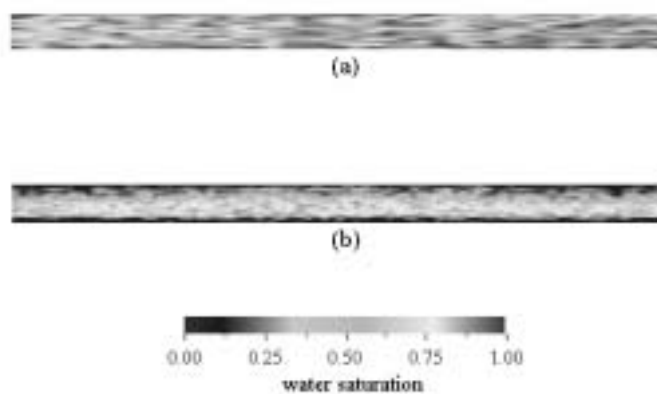
Figure 4. Water saturations obtained from X-ray CT scanning the sand samples: (a) homogeneous case with uniform distribution of water and gas (2 cm slices with 0.2 mm resolution; average water saturation is 90%), and (b) horizontal-patchy case with gas cap along the top (1 cm slices with 0.2 mm resolution; average water saturation is 60%). The length of the image is 81 cm, and the diameter is 4.3 cm.
