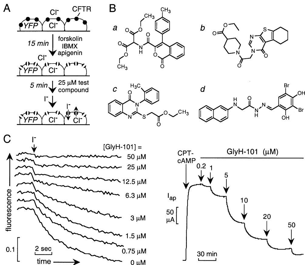
FIGURE 1. Identification of novel classes of CFTR inhibitors by high-throughput screening. (A) Screening procedure. FRT cells coexpressing a halide-sensing yellow fluorescent protein (YFP-H148Q) and human wild-type CFTR were incubated with activating cocktail for 15 min before addition of test compounds at 25 \mu M. Iodide influx was induced by rapid addition of an iodide-containing solution. (B) Structures of novel classes of CFTR inhibitors identified by screening of a collection of 100,000 drug-like small molecules. (C) Dose inhibition of the glycine hydrazone GlyH-101 determined by fluorescence assay (left) and apical \text{Cl}^- current analysis (right). Apical \text{Cl}^- current was induced by 100 \mu M CPT-cAMP. CPT-cAMP and GlyH-101 were added to both apical and basolateral solutions.
