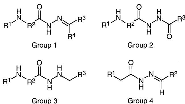
FIGURE 4. General structures of the synthesized compounds. See Table I for list of substituents and CFTR inhibition activities.
