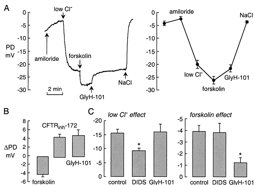
FIGURE 8. GlyH-101 inhibits forskolin-induced hyperpolarization in nasal potential difference in mice. (A, left) Nasal PD recording showing responses to amiloride (100 \mu M) and low \text{Cl}^- (4.7 mM) solutions. Where indicated, the low \text{Cl}^- solutions contained forskolin (10 \mu M) without or with GlyH-101 (10 \mu M). (A, right) Averaged PD values (mean \pm SEM, n = 5 ). (B) Paired analysis of experiments as in A showing PD changes ( \Delta PD) after forskolin (10 \mu M), CFTR inh -172 (20 \mu M), and GlyH-101 (10 \mu M). (C) A series of experiments was done in which all solutions contained DIDS (100 \mu M) or GlyH-101 (10 \mu M). \Delta PD (mean \pm SEM) for low \text{Cl}^- and forskolin-induced hyperpolarizations. *, P < 0.005 for reduced \Delta PD compared with control. CFTR inh -172 data taken from Salinas et al. (2004).
