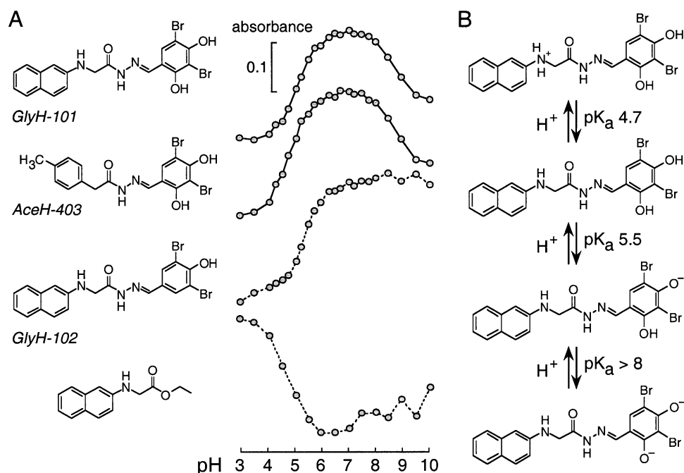
FIGURE 7. Determination of pH-dependent ionic equilibria of GlyH-101 by spectrophotometric titration of GlyH-101 analogues. (A) Chemical structures (left) and corresponding pH-dependent absorbance changes (right) of compounds (10 \mu M) in NaCl (100 mM) containing MES, HEPES, boric acid, and citric acid (each 10 mM) titrated to indicated pH using HCl/NaOH. Absorbance changes measured at wavelengths of 346, 348, 346, and 236 nm (top to bottom). (B) Deduced ionic equilibria of GlyH-101 showing pKa values.
