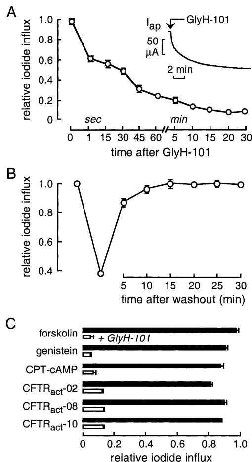
FIGURE 2. CFTR inhibition by the glycine hydrazide GlyH-101. Studies were done in FRT cells coexpressing human wild-type CFTR and a halide-sensing yellow fluorescent protein (YFP). (A) Kinetics of CFTR inhibition. After CFTR stimulation by a mixture of activators (10 \mu M forskolin, 100 \mu M IBMX, 20 \mu M apigenin), iodide influx (mean \pm SEM, n = 3 ) was measured by the fluorescence assay at indicated times after addition of GlyH-101 (10 \mu M). Inset shows reduction in apical \text{Cl}^- current (activated by 100 \mu M CPT-cAMP) after rapid addition of GlyH-101 (5 \mu M). (B) Kinetics of reversal of inhibition after GlyH-101 washout. FRT cells were incubated with the mixture of activators containing 5 \mu M GlyH-101 for 5 min. GlyH-101 was removed and cells were washed three times with PBS. Iodide influx was measured at specified times after GlyH-101 washout in the presence of the activator mixture. (C) Inhibition of iodide influx (mean \pm SEM, filled bars) by GlyH-101 (50 \mu M, open bars) after CFTR stimulation by indicated agonists (all 50 \mu M, except for forskolin 10 \mu M, CPT-cAMP 500 \mu M).
