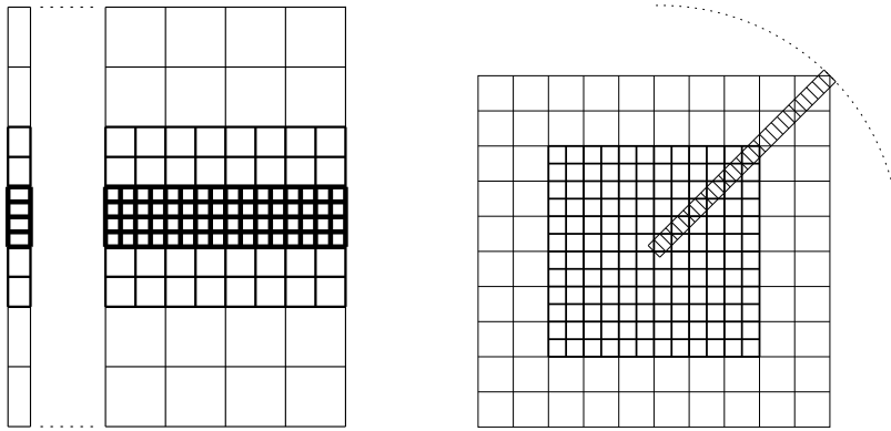
Figure 1. (Left) For multi-level problems in planar geometry, we force a direct alignment between the base state cell centers and the Cartesian grid cell centers by allowing the radial base state spacing to change with space and time. (Right) For multi-level problems in spherical geometry, since there is no direct alignment between the base state cell centers and the Cartesian grid cell centers, we choose to fix the radial base state spacing across levels. Reprinted from Paper V (Nonaka et al. 2010).
