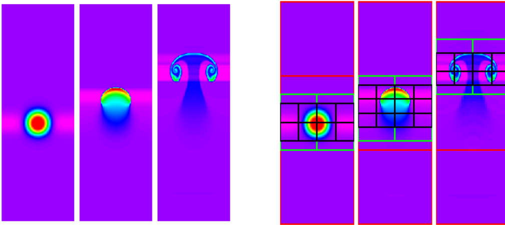
Figure 7. Time-lapse cross-section of a hot bubble in a white dwarf environment at t = 0, 1.25, and 2.5 s for (left) single-level simulation, and (right) adaptive simulation at the same effective resolution. The red, green, and black boxes indicate grids of increasing resolution
