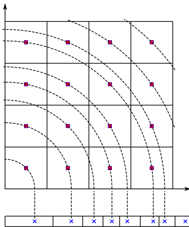
Figure 2. A direct mapping between the base state cell centers (red squares) and the Cartesian grid cell centers (blue crosses) is enforced by computing the average of the grid cell centers that share the same radial distance from the center of the star.
