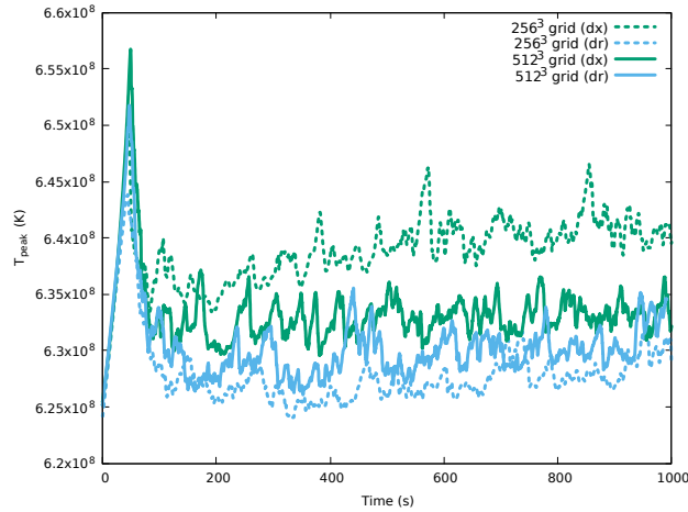
Figure 5. Peak temperature, T_{\text{peak}} in a white dwarf at grid resolutions of 256^3 (dotted line) and 512^3 (solid line) until t = 1000 for uniform ( dx ) and irregular ( dr ) base state spacing. Note that the irregularly-spaced solution agrees better with the uniformly-spaced solution as the resolution increases.
