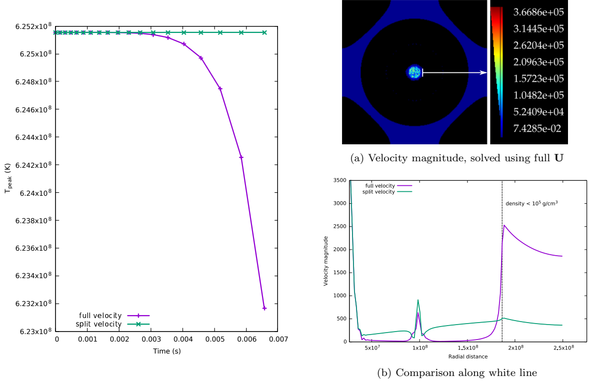
Figure 9. When solving for the full velocity \mathbf{U} in the nodal projection step instead of the split velocity formulation, we illustrate (left) the peak temperature, T_{\text{peak}} in a white dwarf at resolution of 256^3 during the early evolution of the star and (right) the magnitude of velocity at early time. We observe much larger velocities outside the density cutoff region, \rho < 10^5 \text{ g cm}^{-3} , that are not seen when we split the velocity dynamics.
