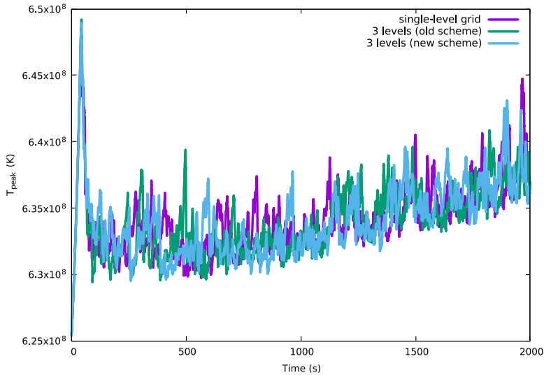
Figure 8. Peak temperature, T_{\text{peak}} , in a white dwarf from t = 0 to 2000 s for grids with effective resolution of 512^3 . We can see that the adaptive grids with two levels of refinement give very similar solution trends compared to the single-level grid.
