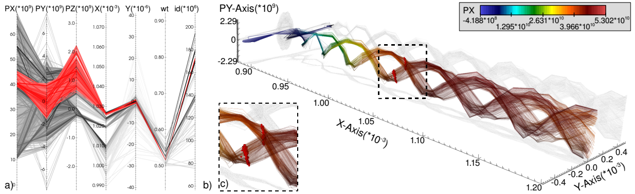
Figure 5: a) Parallel coordinates of time step t = 86 of a particle dataset showing all particles with a momentum in x direction of p_x > 1e10 (gray) and a selected particle beam (red). b) Semi-transparent rendering of the paths of the selected particles over time, using time steps 0 through 105. Color indicates p_x (the momentum in the acceleration direction x ) and height indicates momentum in y direction ( p_y ). The particles of the selected beam at time step t = 86 are shown in addition (red). The transition in color from blue to red along the particle paths shows that the selected particles are constantly accelerated over time. The cork-screw-like structure of the paths illustrates the oscillating motion of the particles in the wake. c) Close-up view of the region in figure b showing the selected particles at time step t = 86 .
