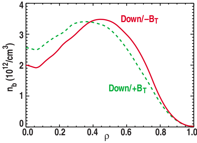
FIG. 16. (Color online) Radial profile of beam ion density for +B_T (dashed line) and -B_T (solid line).
