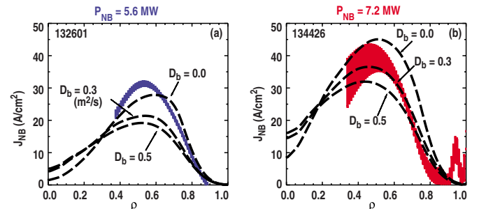
FIG. 19. (Color online) Effects of ad hoc anomalous fast ion diffusion on off-axis NBCD profiles. The measured NBCD profile fits best with the theoretical calculation with D_b=0 and 0.3 \text{ m}^2/\text{s} at (a) P_{NB}=5.6 MW and (b) 7.2 MW, respectively.
