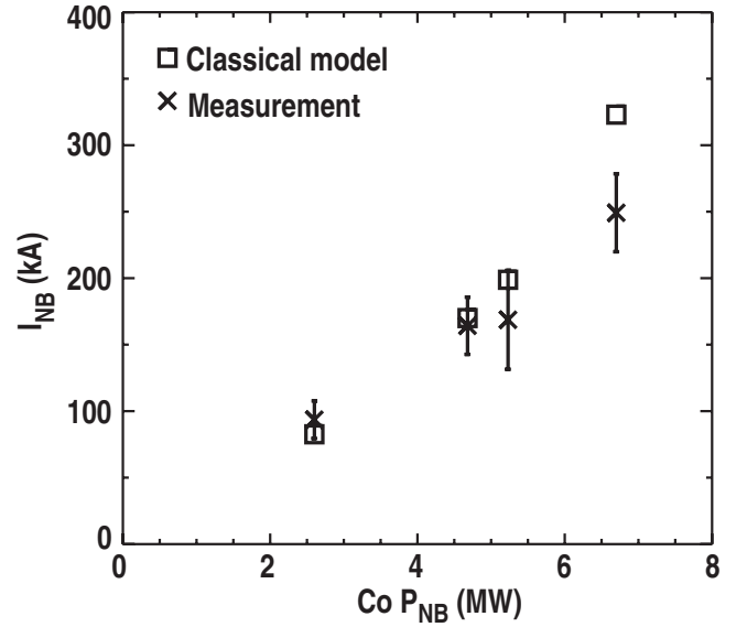
FIG. 18. Comparison of measured NBCD with NUBEAM model with D_b=0 for different injection powers (upshifted plasma with +B_T , favorable alignment configuration)
