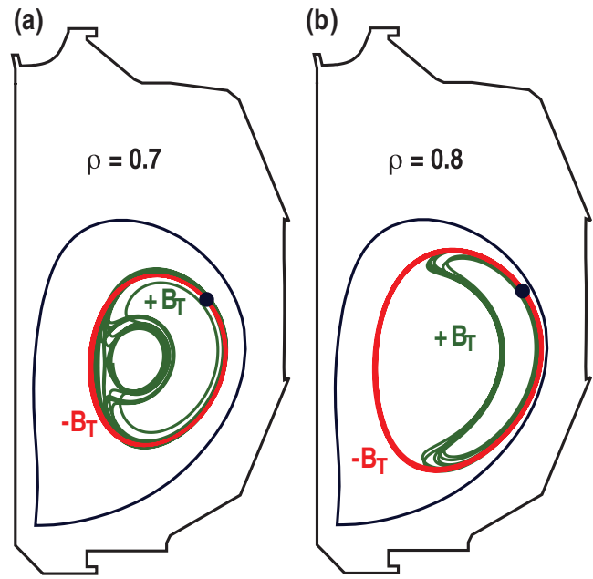
FIG. 14. (Color) Guiding center orbits of beam ions born at the same radial location [(a) \rho=0.7 and (b) \rho=0.8 ] but in the opposite B_T direction (green: +B_T , red: -B_T ).
