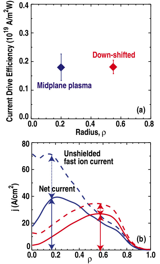
FIG. 7. (Color online) (a) Comparison of measured NBCD efficiency between on- (midplane plasma) and off-axis (downward shifted plasma) injection, (b) profiles of calculated unshielded fast ion current (dashed line), and net NBCD profiles (solid line) for on- and off-axis injection.
