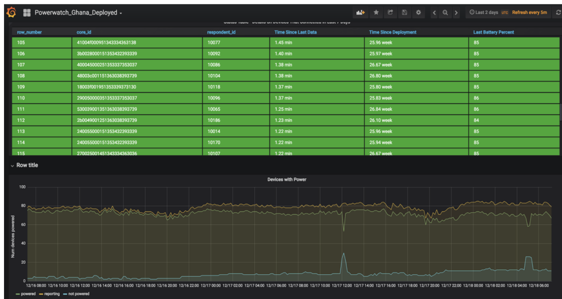
Figure 4.4: Early Engineering Dashboard. This is accessed using a web browser. The table towards the top of the screen lists all sensors, the time since the last data received, the total time it has been deployed, and its current battery life. The bottom graph shows a time series representation of all PowerWatch devices. The orange line is all of the devices. The green line is all devices that believe the power is on. The blue line is all devices that believe the power is off. There are two outages present in this view, which can be seen as a spike in the blue line as more devices report that the power is off and a dip in the green line as less devices report power is on. While not the most aesthetically pleasing, it allowed us to handle medium to large scale deployments.
