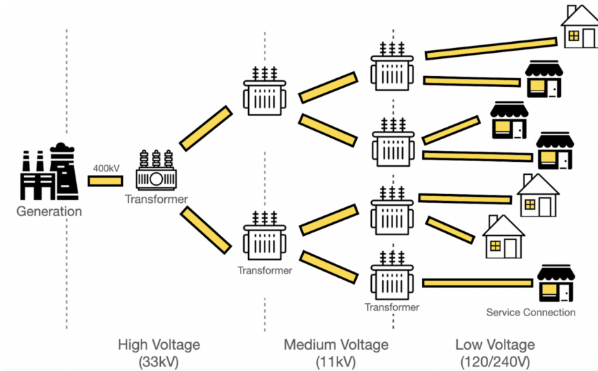
Figure 2.1: Basic model of the grid. In this model we see the grid hierarchy as a function of voltage level. A few high-voltage lines each serve a large section of the grid; then more-numerous medium-voltage feeder lines serve smaller subsections of the grid; and then myriad low-voltage distribution lines serve individual households and businesses through the meter installed at the service connection. This simple model omits details that are less important for our primary sensing methodology including phases, customer segments, and the distinction between transmission and distribution networks.
