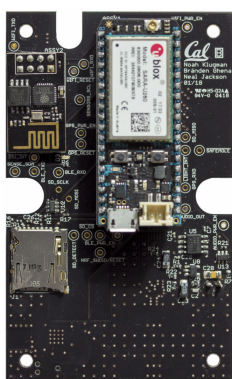
(a) PowerWatch PCB.
