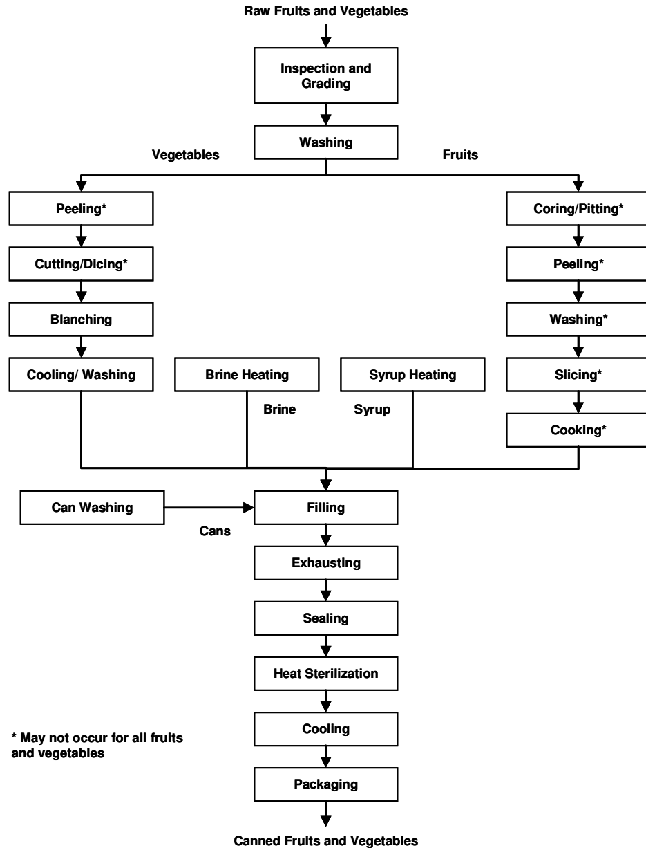
Figure 3.1: Process diagram for fruit and vegetable canning
