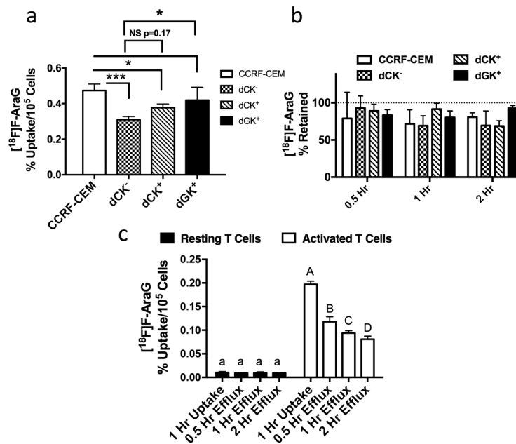
Figure 1. [18F]F-AraG Accumulates in Cells via dCK and dGK Activity and at Increased Levels in Activated Versus Resting Primary Human T Cells a) Uptake and b) retention of [18F]F-AraG across wild-type CCRF-CEM T lymphoblasts, mutant CCRF-CEM dCK - cells (dCK - ), and dCK - cells overexpressing either dCK (dCK + ) or dGK (dGK + ) (n=4 per cell type per time point). Significantly less uptake was seen due to the loss of dCK in wild-type cells (CCRF-CEM vs. dCK - ), (p<0.001). There was a trend towards higher uptake in dCK + versus dCK - cells, whereas dGK + cells had significantly higher uptake compared to dCK - cells and equivalent uptake compared to wild-type cells. No differences in retention were seen across cell types. c) Activated primary human T cells had significantly higher [18F]F-AraG uptake compared to resting T cells at all time points examined (**p<0.001; n=4 per cell state per time point). Data in all graphs are expressed as mean ± SD.
