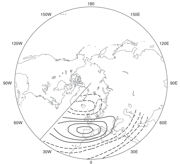
FIG. 7. Leading EOF of the zonal wind response over the domain 42^{\circ}\text{W} – 60^{\circ}\text{E} contoured at 0.02 with negative values dashed and the zero contour suppressed. The meridian at 42^{\circ}\text{W} is indicated to facilitate comparison with Fig. 3.
