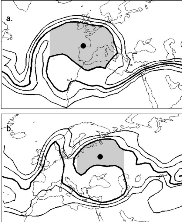
FIG. 2. (a) An example of anticyclonic Rossby wave breaking on 25 Dec in the second member of the control ensemble. Circumpolar contours of potential vorticity are shown at 1-PVU increments, with the 4-PVU contour being thick. The poleward tongue associated with the depicted instance of anticyclonically overturning PV has its area shaded and its centroid marked by a filled circle. (b) As in (a), but for a case of cyclonic Rossby wave breaking on 8 Mar in the 28th member of the control ensemble, with the 6-PVU contour being thick.
