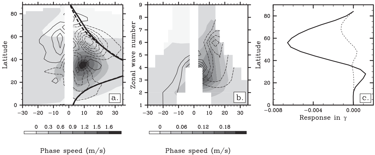
FIG. 4. (a) Eddy momentum flux decomposed by latitude and phase speed for December–January in the control ensemble (shading; \text{m}^2 \text{s}^{-2} ), and the model response for the same field (thin contours at 0.015 \text{ m}^2 \text{s}^{-2} with negative values dashed and the zero contour suppressed). The thick solid (dashed) curve shows the zonally averaged zonal wind for the control (forced) ensemble. (b) Results from 55^\circ\text{N} in (a) transformed into zonal wavenumber–phase speed space with response curves contoured at 5 \times 10^{-3} \text{ m}^2 \text{s}^{-2} . (c) Zonally averaged response in the relative frequency of anticyclonic (thick) and cyclonic (dashed) Rossby wave breaking for the entire duration of the experiment.
