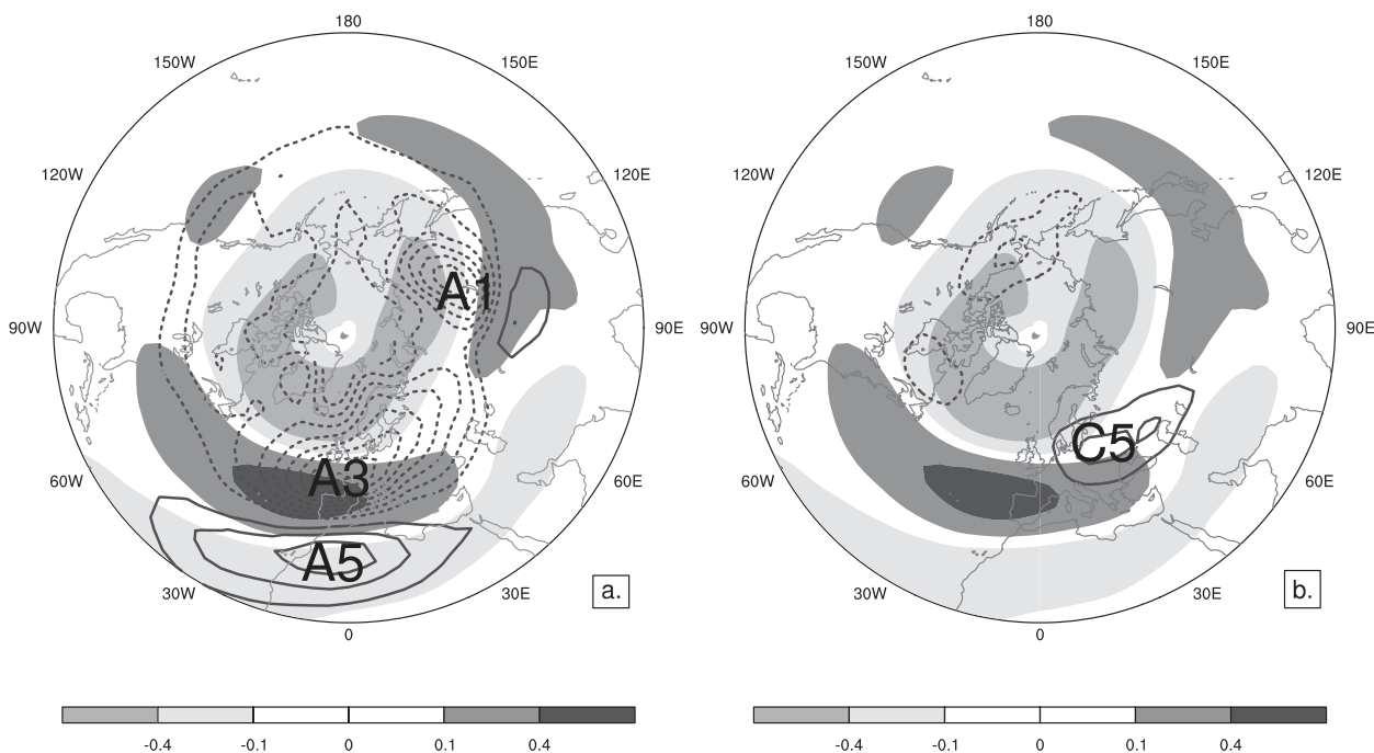
FIG. 5. (a) The response in anticyclonic Rossby wave breaking relative frequency \delta\gamma_a contoured at 2 \times 10^{-3} with negative values dashed and the zero contour suppressed. Shading shows the basic pattern of the zonal wind response in Fig. 3b. (b) As in (a), but for cyclonic Rossby wave breaking \delta\gamma_c . The labeled regions are discussed in the text.
