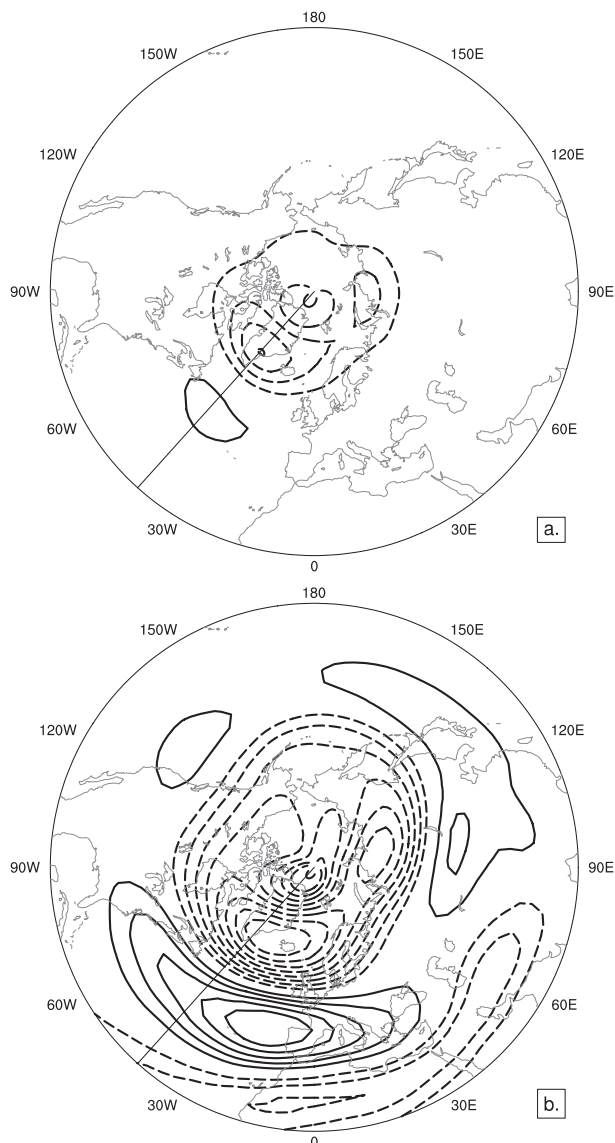
FIG. 3. (a) Response in zonal wind on the 350-K surface averaged over days 1–14 ( \delta u_{1-14} ) contoured at 0.1 \text{ m s}^{-1} with negative values dashed and the zero contour suppressed. (b) As in (a), except averaged over days 15–151 ( \delta u_{15-151} ). The meridian at 42°W is indicated in each panel.
