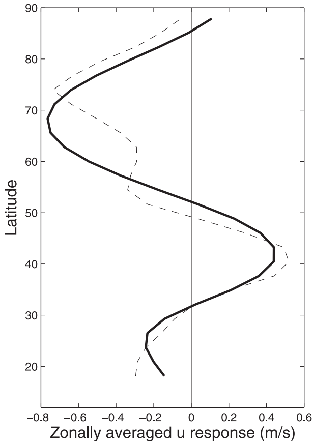
FIG. 6. Zonal average of the zonal wind response from Fig. 3b (thick curve) and a model constructed from the zonal wind forcing patterns of Rossby wave breaking (dashed curve). Additional details on are given in section 3b.
