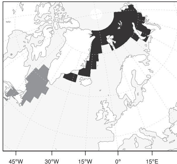
FIG. 1. The sea ice anomalies for mid-January used in the ICE experiment, where black (gray) shading corresponds to ice removal (addition).
