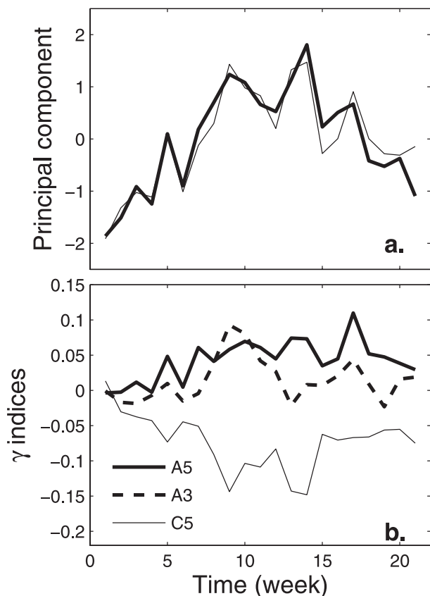
FIG. 8. (a) The principal component associated with the zonal wind response EOF in Fig. 7 (thick) and a model constructed from indices representing the response in Rossby wave breaking (thin curve). (b) The Rossby wave breaking response indices used to develop the model in (a). Additional details are given in the text.
