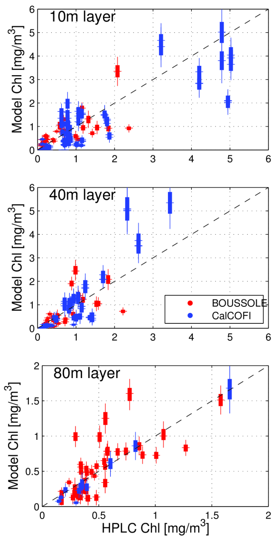
Figure 1.8: Comparison of model-returned chlorophyll values versus chlorophyll values for BOUSSOLE (red) and CalCOFI (blue), for each of 10m (top), 40m (middle), and 80m (bottom). The spread in the y-direction derives from the Monte-Carlo handling of error; this is a compilation of 200 runs with random numbers used to handle errors in the various modules. The thick lines represent the 68% distribution, while the thin lines represent the 95% distribution.
