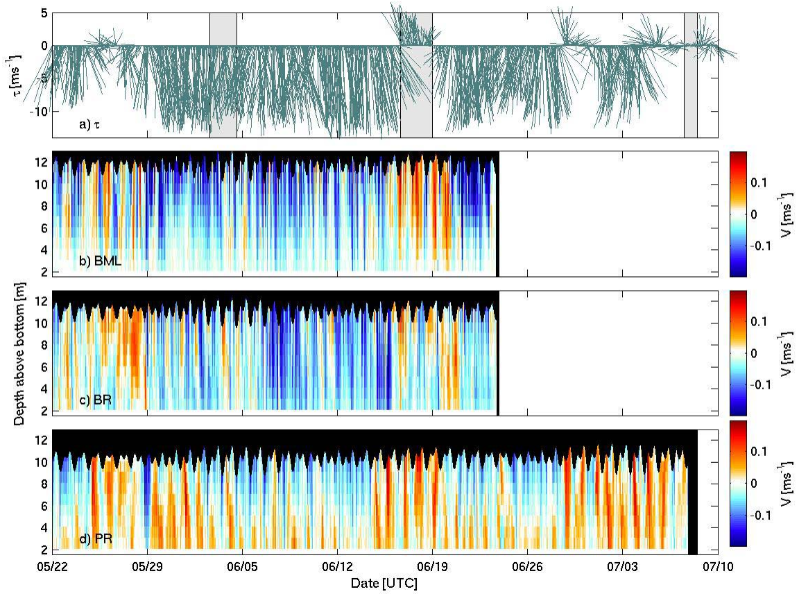
Figure 6. Time series of a) wind ( \text{ms}^{-1} ) at NDBC 46013 and alongshore current ( \text{ms}^{-1} ) at b) Bodega Marine Lab (BML), c) Bodega Rock (BR) and d) Pinnacle Rock (PR). For the current plots the y-axis represents distance above the bottom and the black shading in each panel represents the sea surface elevation obtained from the pressure recorded by the bottom-mounted ADCP. As for the wind time series, positive (red) velocities are directed poleward in the alongshore direction.
