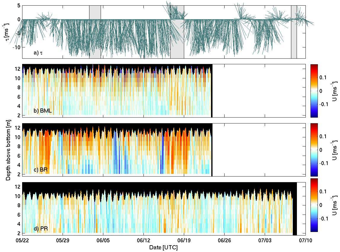
Figure 7. As for Figure 6 but the current velocities are in the across-shore direction.
