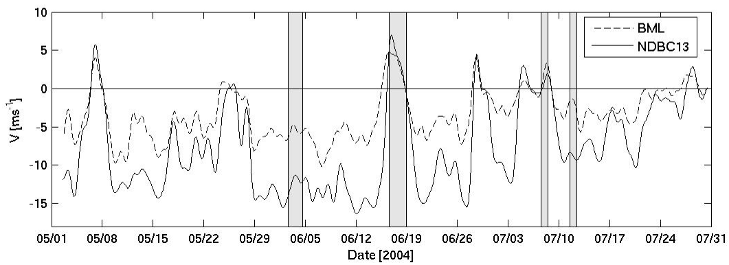
Figure 2. Time series of alongshore wind ( \text{ms}^{-1} ) at BML (dashed) and NDBC 46013 (solid). The gray bars represent the 4 survey periods; upwelling, downwelling, relaxation, and incipient upwelling respectively.
