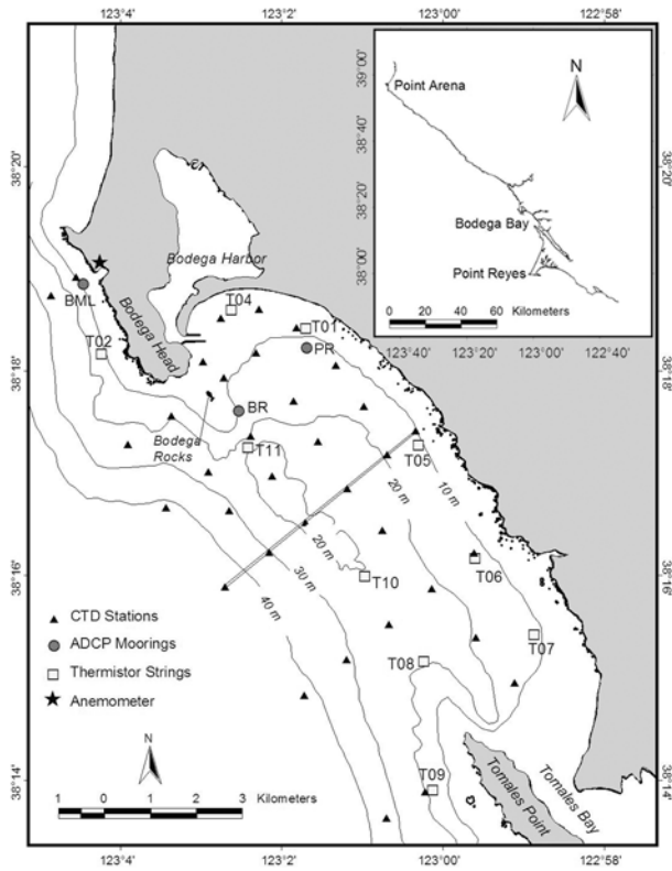
Figure 1. Map showing the location of the 30 CTD stations (triangle), 3 ADCP moorings (circle) and 10 thermistor strings (square). The straight black line represents a CTD transect within Bodega Bay and the light black lines are the bathymetric contours. The inset shows the location of Bodega Bay north of Pt Reyes on the west coast of the USA.
