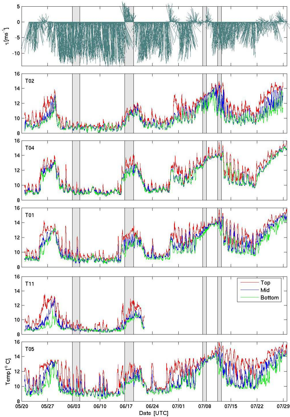
Figure 3. Top Panel: Hourly vectors of wind velocity ( \text{ms}^{-1} ) from NDBC 46013 where positive values are alongshore poleward. Lower Panels: time series of temperature ( ^{\circ}\text{C} ) in the northern half of Bodega Bay at three depths; 1 m off the bottom (approximately 14 m); mid water column (approximately 8 m); and 1 m below the surface. Shaded areas represent the timing of the four hydrographic surveys.
