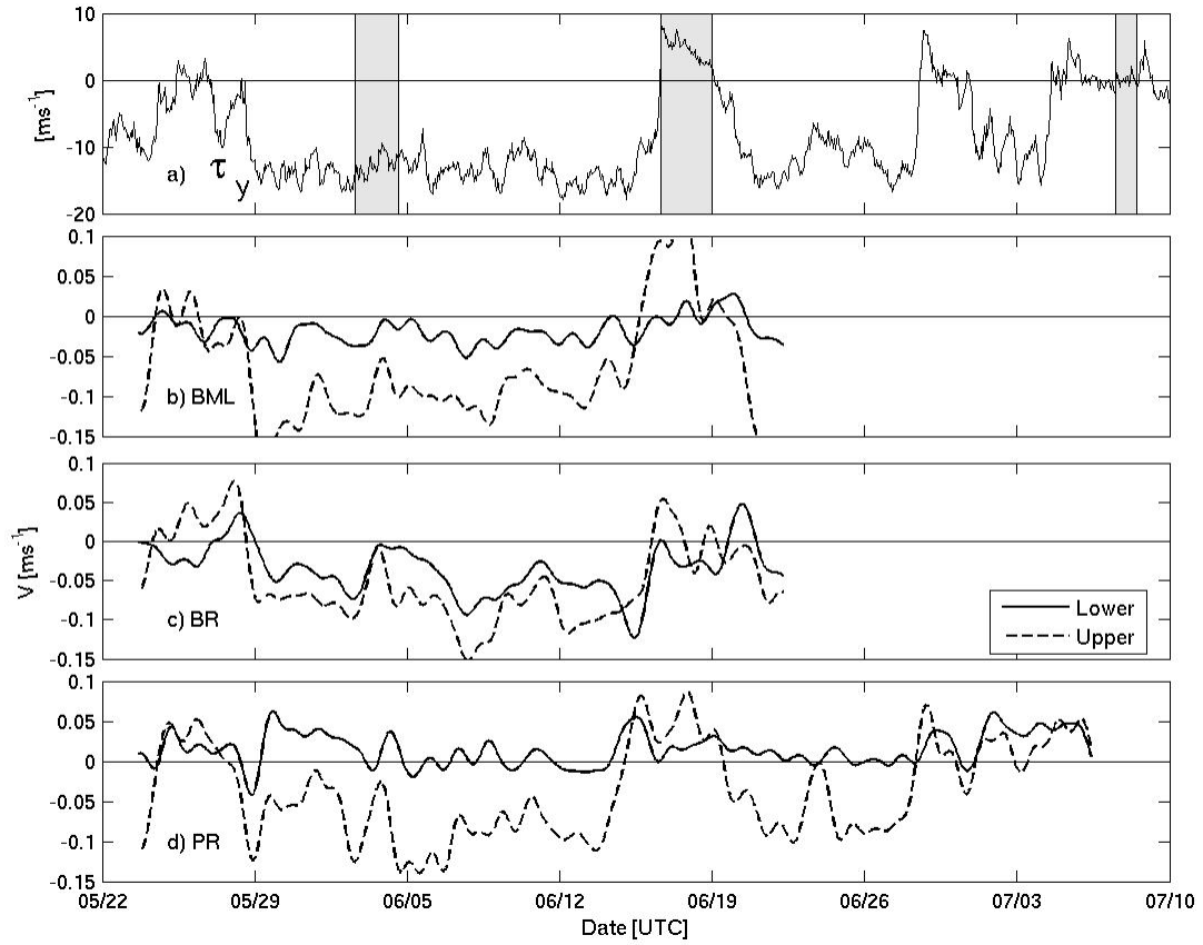
Figure 8. a) Alongshore component of wind ( \text{ms}^{-1} ), and depth averaged, sub-tidal, alongshore velocity at BML, BR and PR (b-d) respectively. Depth averaged velocities are calculated for an upper layer (8-10 m above the bottom) and a lower layer (2-6 m above the bottom).
