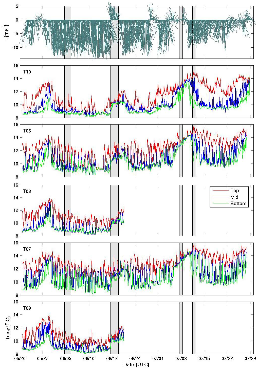
Figure 4. As for Figure 3 for the thermistors in the southern half of Bodega Bay.
