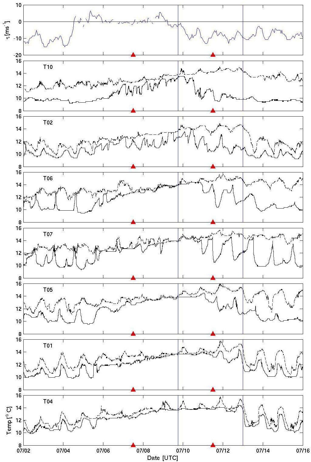
Figure 5. Top panel shows alongshore component of wind velocity ( \text{ms}^{-1} ). Lower panels show temperature time series ( ^{\circ}\text{C} ) at each of the thermistor moorings sub-surface (dashed) and at the bottom (solid). The vertical lines delineate the timing of an upwelling event and the associated cooling of bottom waters. The triangles represent the timing of the hydrographic surveys.
