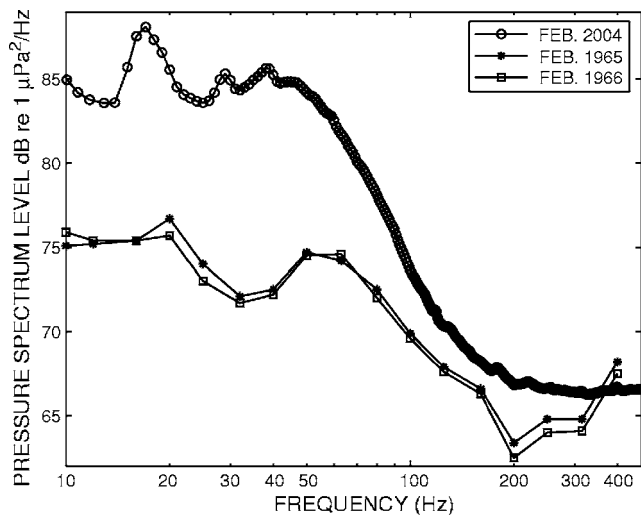
FIG. 3. Sound pressure spectrum levels (1 Hz bins) for the month of February 2004 compared to February 1965 and 1966. During February blue whales are absent from this site and the peak near 17 Hz in 2004 is from fin whale calls.
