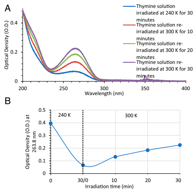
Fig. 2. (A) Absorption spectrum of thymine solution irradiated with 254-nm light at 240 K and reirradiated at 300 K for 10, 20, and 30 min. (B) Change in OD at 263.8 nm, after UV irradiation at 240 K followed by irradiation at 300 K, as a function of irradiation time (minutes).
