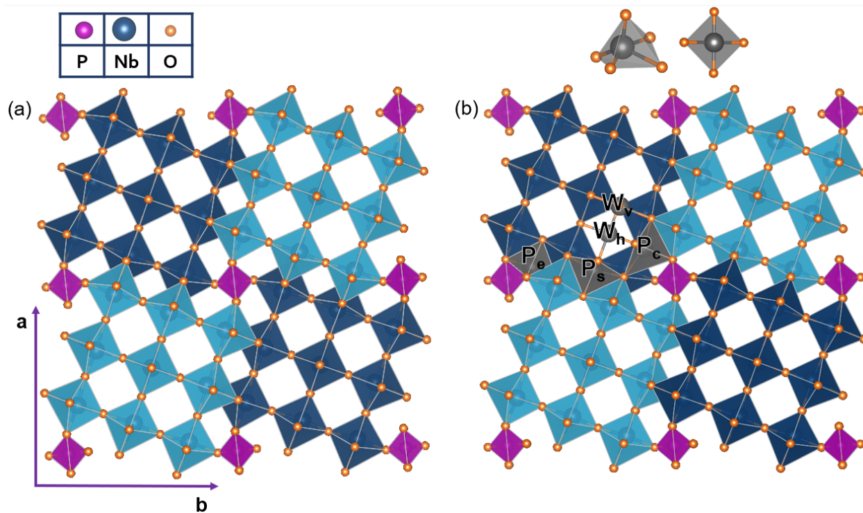
Figure 1: (a) The crystal structure of \text{PNb}_9\text{O}_{25} as viewed down the c axis. The octahedra correspond to \text{NbO}_6 , the tetrahedra correspond to \text{PO}_4 . (b) The pyramidal and square polyhedra show one example of each symmetrically distinct lithium site.
