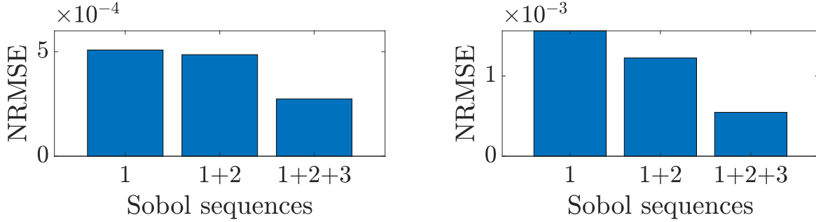
FIG. 10: Mean of NRMSE for test data when the machine learning model is trained using Sobol sets. (Left) Error bars for \rho , (Right) Error bars for b .
