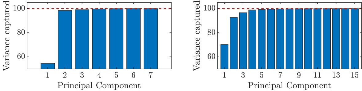
FIG. 5: Cumulative percentage of variance vs Principal components for \rho ( left ) and b ( right ). The red dashed line shows 99.99% variance.
