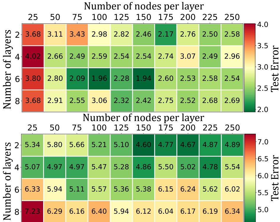
FIG. 12: (Top) Test error ( \times 10^{-5} ) for various architectures of \mathcal{N}_1 (trained for \rho ), (Bottom) Test error ( \times 10^{-4} ) for various architectures of \mathcal{N}_2 (trained for b ).
