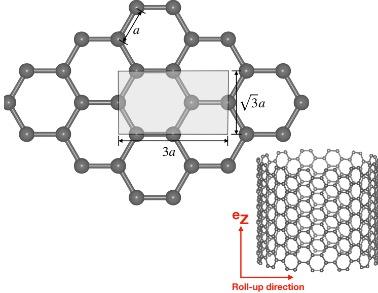
FIG. 1: Roll-up construction of an undeformed armchair carbon nanotube, starting from a graphene sheet. The 4 atoms shown in the shaded region are used for the data generation process using Helical DFT. The parameter a represents the planar interatomic distance of 1.407 Angstrom.
