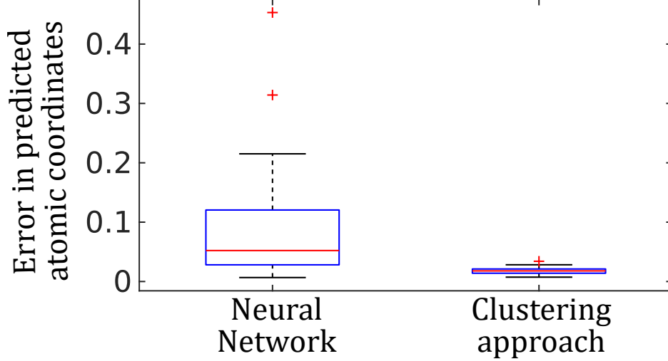
FIG. 13: Error in predicted atomic coordinates (in Bohr), i.e., the distance between true and predicted nucleus positions, using a neural network and the DBSCAN based clustering approach.
