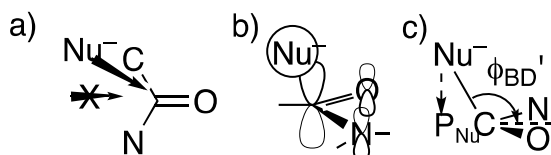
Figure 2. Approach of a nucleophile to an amide carbonyl. (a) Top view of approach anti to both O and N of an amide. (b) Overlap between the orbital on \text{Nu}^- and the amide \pi^* MO. (c) Side view of modified Bürgi-Dunitz angle.
