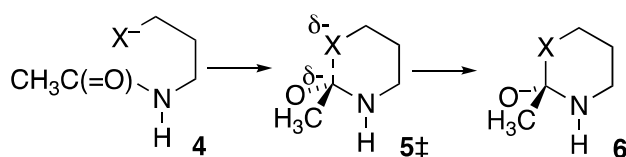
Scheme 3. Cyclization of homologous N -CH 2 CH 2 CH 2 X - -substituted acetamides ( X=O or S ).
