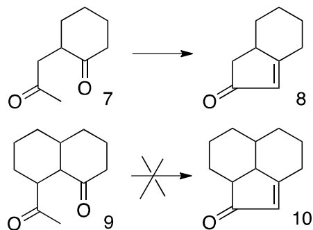
Scheme 4. Constraint on aldol condensation.
