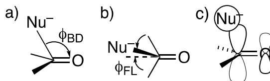
Figure 1. Approach of a nucleophile to a ketone or aldehyde carbonyl. (a) Side view of Bürgi-Dunitz angle. (b) Top view of Flippin-Lodge angle. (c) Overlap between the orbital on \text{Nu}^- and the \pi^* MO of C=O.
