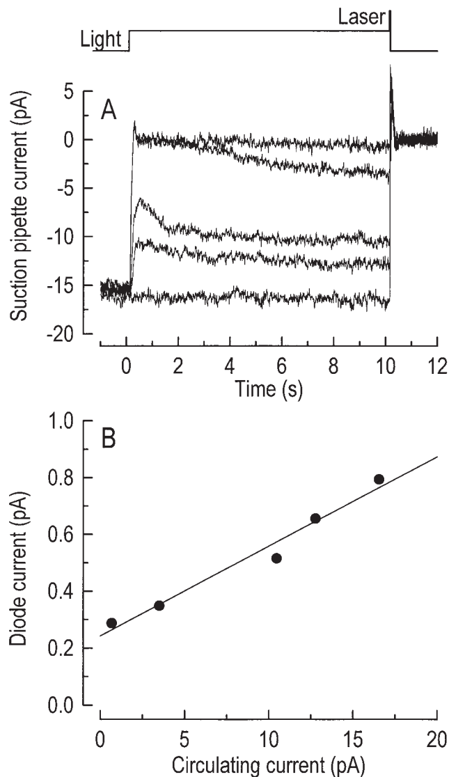
FIGURE 5. Determination of the relationship between steady state circulating current and outer segment Ca^{2+} concentration. (A) Suction pipette current records in response to stimulation with 10 s of background illumination followed by a 20-ms laser pulse, during which fluo-3 fluorescence was measured. Steady light stimuli of wavelength 500 nm delivered 0, 3,640, 13,000, 171,000, and 2,520,000 photons per \mu m^{-2} s^{-1} in this cell. The cone outer segment was exposed to an ethanolic solution containing 50 \mu M 11-cis-retinal throughout the experiment. The extent of photopigment regeneration between laser exposures was assessed by the recovery of both the amplitude and response waveform of a saturating flash of wavelength 570 nm. The top trace is the laser light monitor. (B) Photodiode current measured during laser illumination plotted against the amplitude of the circulating current after it had reached steady state in the presence of the background. The data were fitted with a regression line using a least-squares algorithm.
