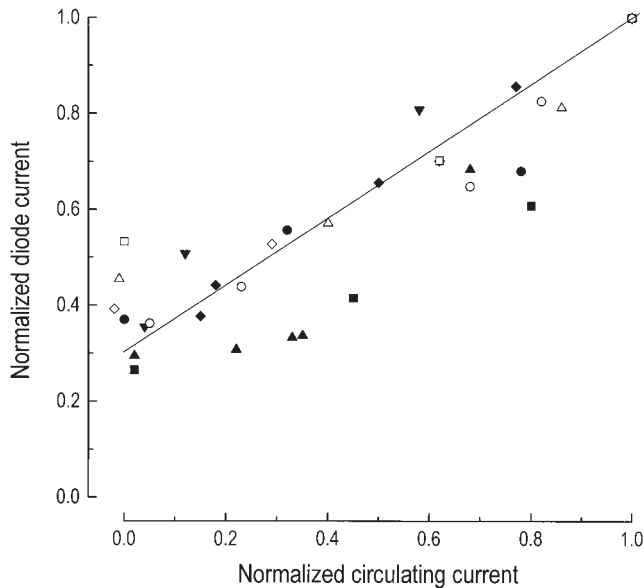
FIGURE 6. Collected results from nine experiments to determine the relationship between steady state circulating current and fluo-3 fluorescence. Data have been normalized according to the circulating current and fluo-3 fluorescence in darkness to allow comparison between cells. Normalized diode current has been plotted against the fraction of circulating current that remained after exposure to background illumination. The data have been fitted with a regression line constrained to pass through unity by a least-squares algorithm.
