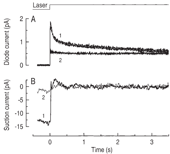
FIGURE 2. Simultaneous measurements of fluo-3 fluorescence and circulating current from a blue-sensitive cone during a 7-s laser exposure. (A) Fluo-3 fluorescence signal excited by the laser spot and recorded by the photodiode. (B) Circulating current measured by the suction pipette in response to the laser exposure. In each case, 1 represents the first exposure of the dark-adapted cone to the laser spot and 2 shows the response to a second laser exposure 10 s later. The time axis has been truncated to show the initial 3.5 s of the laser exposure for ease of comparison with the data of Fig. 1. The light-induced decline in fluo-3 fluorescence (A, 1) could be fitted with the sum of two exponentials with time constants of 90 and 2,300 ms using a least-squares algorithm. The top trace is the laser light monitor.
