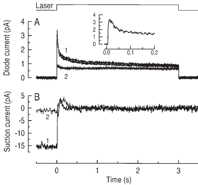
FIGURE 1. Simultaneous measurements of fluo-3 fluorescence and circulating current from a red-sensitive cone during a 3-s laser exposure. (A) Fluo-3 fluorescence signal excited by the laser spot and recorded by the photodiode. (B) Circulating current measured by the suction pipette in response to the laser exposure. In each case, 1 represents the first exposure of the dark-adapted cone to the laser spot and 2 shows the response to a second laser exposure 10 s later. The light-induced decline in fluo-3 fluorescence (A, 1) could be fitted with the sum of two exponentials with time constants of 27 and 430 ms using a least-squares algorithm. The residual decline in fluo-3 fluorescence seen at the onset of the second laser exposure (A, 2) is likely to correspond to the small recovery in circulating current that had taken place at that time (B, 2). The initial peak in the suction pipette recording (B) is likely to represent contamination of the photoresponse by voltage-sensitive conductances in the cone inner segment (Barnes and Hille, 1989). The top trace is the laser light monitor. (Inset) The fall in fluo-3 fluorescence during the first 200 ms with the same exponential fit as described above.
