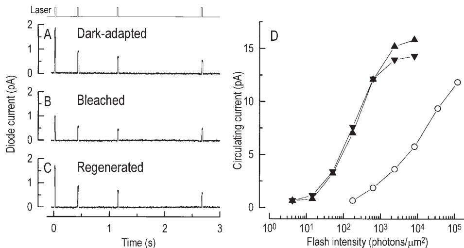
FIGURE 4. Changes in outer segment \text{Ca}^{2+} concentration and flash sensitivity for a red-sensitive cone during the photopigment cycle. (Left) Fluo-3 fluorescence measurements (A) in the dark-adapted cone, (B) after laser-induced photopigment bleaching, and (C) after photopigment regeneration with an ethanolic solution containing 50 \mu\text{M} 11-cis-retinal. (Top) Laser light monitor; laser illumination delivered as a sequence of four 20-ms pulses over a 3-s period. (D) Response-intensity relationships for the cone in the dark-adapted state ( \blacktriangle ), after bleaching by the laser ( \circ ), and after regeneration of the photopigment ( \blacktriangledown ). The response-intensity relation was determined by delivering a series of flashes of increasing intensity before each fluorescence measurement. Each point is the average of four flash responses.
