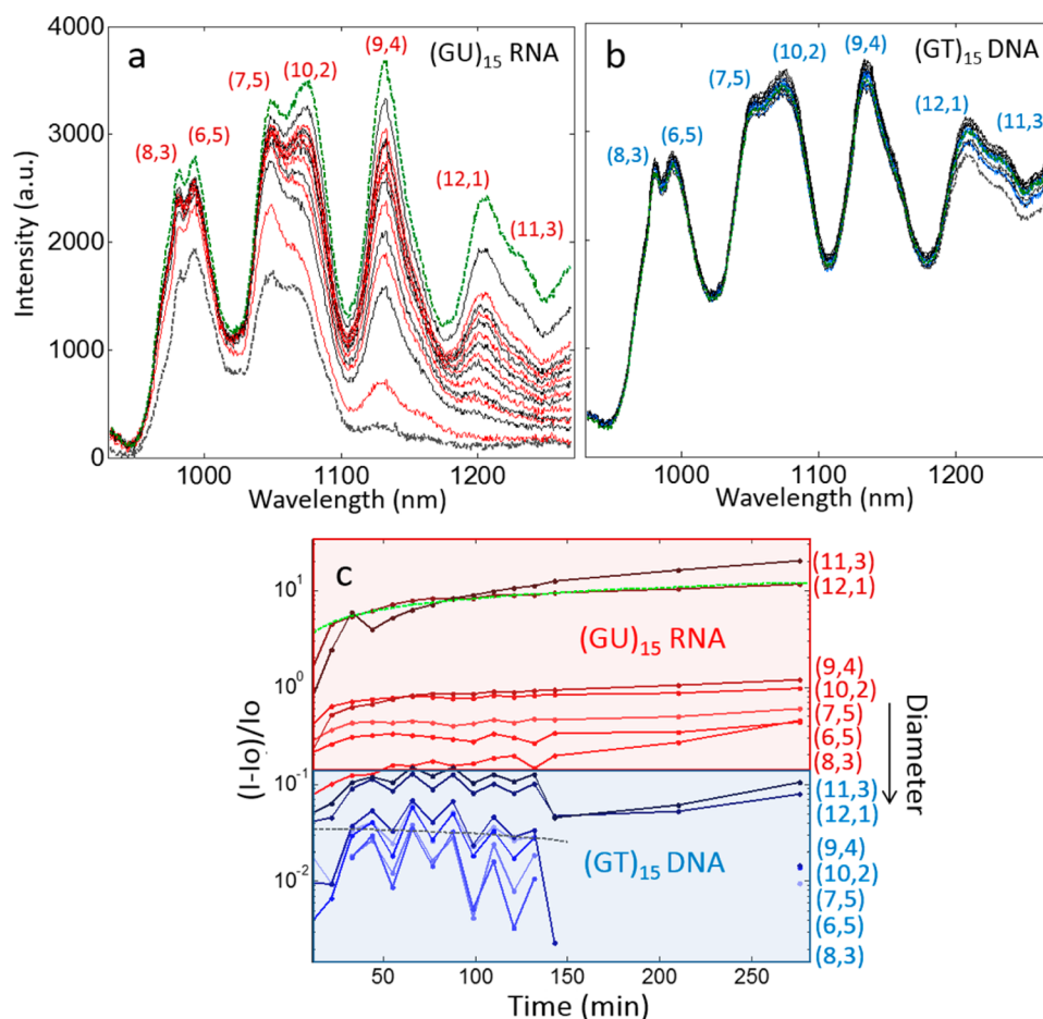
Figure 1. DNA and RNA polymer conformational stability is monitored with increasing SWCNT fluorescence. Fluorescence emission spectra of 1 mg/L (a) (\text{GU})_{15} RNA-SWCNT and (b) (\text{GT})_{15} DNA-SWCNT over the course of 275 min, with 785 nm, 200 mW excitation source, and 10 s exposure time. Each peak corresponds to the emission of a particular SWCNT chirality from a multichirality SWCNT sample, where the first and last spectra are highlighted as dashed gray and dashed green, respectively. (c) Emission peak for each SWCNT chirality normalized to the initial intensity for (\text{GT})_{15} DNA-SWCNT (blue) and (\text{GU})_{15} RNA-SWCNT (red) over the same time-course. The data for the (7,6) SWCNT chirality for (\text{GU})_{15} RNA-SWCNT (green dashed line) and (\text{GT})_{15} DNA-SWCNT (gray dashed line) is fit by a kinetic model described in the manuscript text. Each plotted line is labeled by the corresponding SWCNT chirality. SWCNT diameter decreases from top to bottom of each of the DNA (blue) and RNA (red) regions of the graph.
