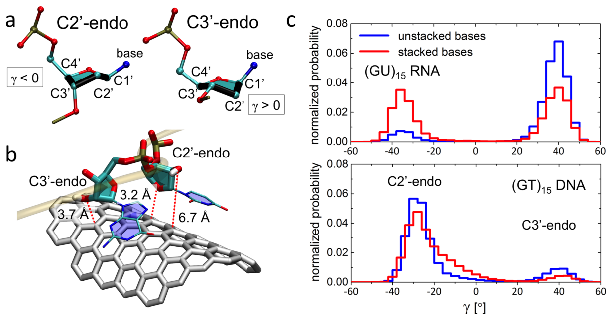
Figure 6. Sugar conformations in nucleic acid strands interacting with SWCNTs. (a) A scheme of C2'-endo and C3'-endo sugar conformations, commonly observed in B-form DNA and A-form DNA/RNA, respectively. The sugar conformation can be characterized by the dihedral angle \gamma (C4'-C3'-C2'-C1'), which is highlighted in black bond representation; \gamma < 0^\circ in the C2'-endo conformation, and \gamma > 0^\circ in the C3'-endo conformation. (b) A representative simulation snapshot of RNA backbone and sugar rings when RNA bases are stacking to the SWCNT. 2'-OH group of the RNA nucleotide can point toward the SWCNT surface (C3'-endo conformation of the sugar ring) or away from the SWCNT surface (C2'-endo conformation; O4' oxygen points to the SWCNT surface). In (a, b), SWCNT atoms are shown in light gray, and nucleic acid atoms are shown in teal (C), red (O), tan (P), blue (N), and white (H) colors. The transparent yellow line shows RNA backbone in tube representation. (c) Histogram distributions of the angle \gamma , shown separately for bases that are stacked on SWCNT and bases that are not stacked on SWCNT. Histogram distributions are obtained from complete (250 ns) simulations of (GT) 15 DNA-SWCNT and (GU) 15 RNA-SWCNT systems.
