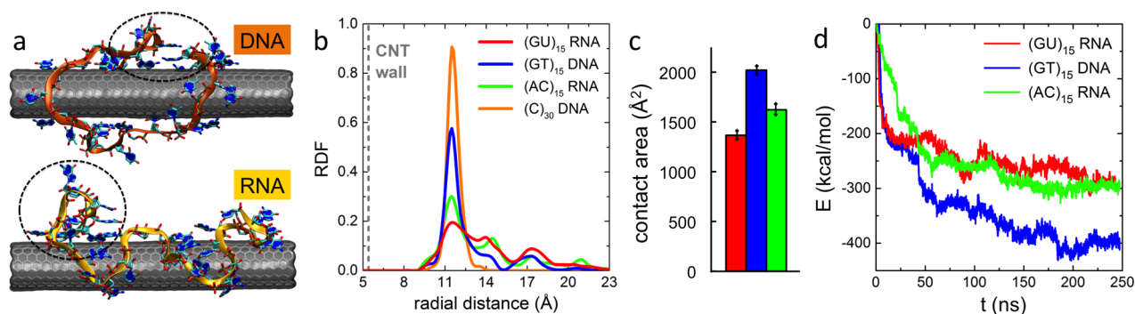
Figure 5. Molecular dynamics of DNA and RNA binding to SWCNT. (a) Snapshots of SWCNT and single (GT) 15 DNA and (GU) 15 RNA strands at the end of 250 ns MD simulations. SWCNT is shown in charcoal, nucleic acid strands are shown in licorice representations, and polynucleotide phosphate backbones are highlighted in orange or gold. Water and ions are not shown for clarity, though have an increased proximity to SWCNT when nucleotides desorb from the SWCNT surface. Nucleic acid atoms are shown in teal (C), red (O), tan (P), and blue (N) colors. (b) Radial distribution of phosphate groups (P atoms) of nucleic acid strands at distance r from the central axis of SWCNT, evaluated for the last 100 ns of simulations. (c) Contact areas between SWCNT and nucleic acid strands, averaged over the last 100 ns of simulations. (d) Interaction energies between SWCNT and nucleic acid strands (including van der Waals contributions; Coulombic contributions are null due to SWCNT atoms having no partial charges, q_{CA} = 0 e). The plots shown in (b–d) are representative of the subset of possible nucleic acid configurations, captured in the performed MD simulations.
