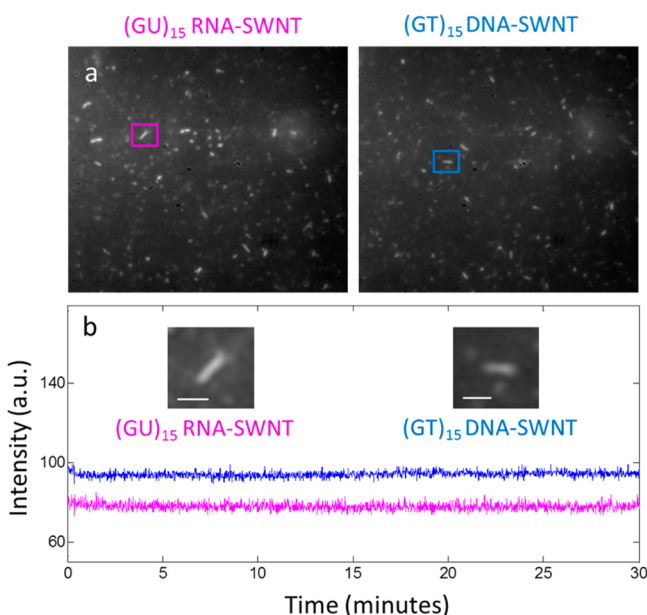
Figure 4. Single-SWCNT imaging of (GU) 15 RNA-SWCNT and (GT) 15 DNA-SWCNT fluorescence stability. (a) Surface-immobilized (GU) 15 RNA-SWCNT and (GT) 15 DNA-SWCNT within a microfluidic channel can be individually monitored for 30 min. (b) Representative individual (GU) 15 RNA-SWCNT (purple) and (GT) 15 DNA-SWCNT (blue) intensities over the course of 30 min, at 785 nm 200 mW excitation, and 1 s exposure time. Scale = 1 \mu m.
