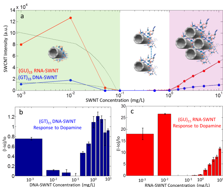
Figure 3. Experimental concentration-dependent fluorescence intensity of DNA and RNA-SWCNT samples, and sensor response. (a) Intensity of (GT) 15 DNA-SWCNT (blue) and (GU) 15 RNA-SWCNT (red) as a function of SWCNT concentration from 10^{-3} to 10^1 mg/L. In the low-concentration regime (below 10^{-1} mg/L, green shaded region), SWCNT fluorescence is dominated by high-intensity emitters resulting from strong stacking of DNA or RNA nucleotides on the SWCNT surface. In the high-concentration regime (above 10^0 mg/L SWCNT, purple shaded region), SWCNT fluorescence is dominated by large quantities of low-intensity polynucleotide-SWCNT complexes. The intermediate concentration range ( 10^{-1} to 10^0 mg/L SWCNT, unshaded region) shows primarily loose-nucleotide stacking species for which the concentration is too low to detect SWCNT emitters. (b) The fluorescence response, (I - I_0)/I_0 , to 100 \mu M dopamine for these same dilutions of (GT) 15 DNA-SWCNT and (c) (GU) 15 RNA-SWCNT at 1130 nm.
