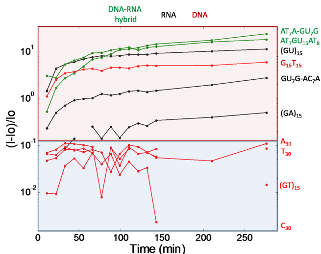
Figure 2. Analysis of DNA, RNA, and DNA-RNA polymer hybrids for conformational stability on SWCNT. Emission peak for (9,4) chirality SWCNT at 1133 nm, normalized to the initial sample intensity for ten different polynucleotide corona phases comprised of DNA (red), RNA (black), or DNA-RNA hybrid (green) sequence variants. Nucleotide polymer stability is similarly high across DNA sequences (blue shaded region) and lower for RNA or DNA-RNA hybrid sequences (red shaded region). A notable exception is \text{G}_{15}\text{T}_{15} DNA, which is known to form secondary G-quadruplex structures, 52 and is expected to form such secondary structures off the SWCNT surface.
