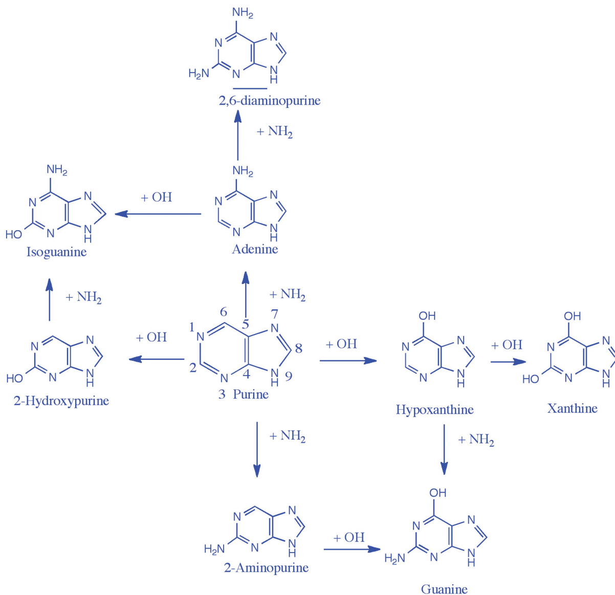
Figure 1. A reaction scheme indicating the amino and hydroxyl group substitutions on the purine ring. Horizontal arrows indicate hydroxyl group substitutions, while the vertical arrows indicate amino group substitutions. Quantum chemical calculations indicate 2-hydroxypurine and adenine are the most favorable singly substituted photo-product, and xanthine, isoguanine, guanine and 2,6-diaminopurine are the most favorable doubly substituted photo-products.
