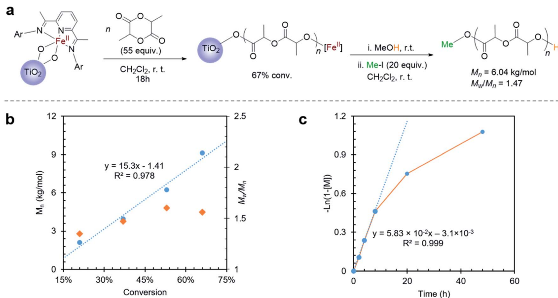
Fig. 2 (a) Reaction scheme for lactide polymerization on \text{Fe(II)}-\text{TiO}_2 particles; kinetic analysis of the lactide polymerization on \text{Fe(II)}-\text{TiO}_2 particles: (b) evolution of M_n versus conversion, M_w/M_n was shown in the second y axis on the right, and (c) first order kinetic plot of lactide polymerization.
