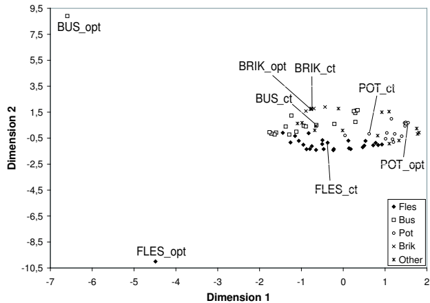
Figure 2: 2-dimensional MDS representation of the bottles. FLES_{ct} , BUS_{ct} , POT_{ct} and BRIK_{ct} represent the central tendencies for fles , bus , pot and brik . FLES_{opt} , BUS_{opt} , POT_{opt} and BRIK_{opt} represent the optimal prototypes for fles , bus , pot and brik .
