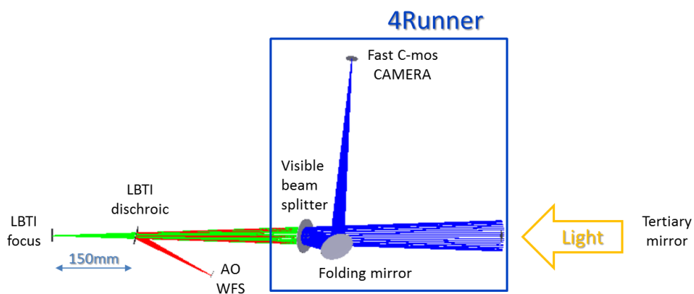
Figure 4. Zemax layout of the 4Runner's optical configuration.
