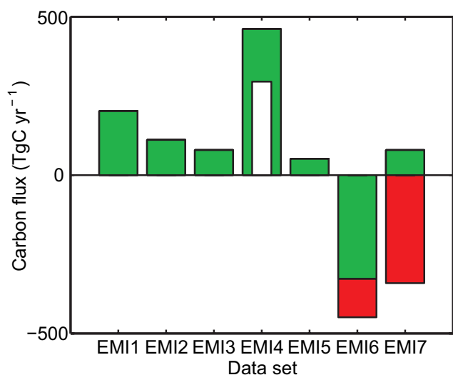
Fig. 6. Comparison of terrestrial carbon fluxes ( \text{TgC yr}^{-1} ) for each land-use activity for Brazil in the 1990s. The white color represents the pasture conversion when pasture is separated from LUCF. The green color shows total LUCF. The red color denotes the biospheric response due to \text{CO}_2 fertilization and climate change.
