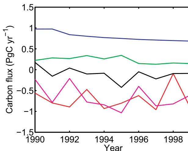
Fig. 7. Interannual variability in LUCF emissions for EMI4 (blue), EMI5 (green) and terrestrial carbon fluxes ( \text{PgC yr}^{-1} ) for EMI6 (red), EMI7 (magenta) and EMI8 (black) for Latin America.
