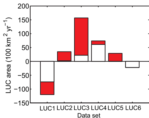
Fig. 1. Comparison of the global sum of land-use change areas in forested areas ( 10^2 \text{ km}^2 \text{ yr}^{-1} ) due to crop and pasture land conversions over the 1990s. The negative (-) signs indicate the decreases in forests areas to crop and pasture land and positive (+) signs represent the increases in forests areas from crop and pasture land. The white color represents the crop land conversion. The red color shows the pasture land conversion.
