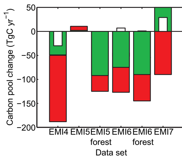
Fig. 4. Comparison of carbon stock changes ( \text{TgC yr}^{-1} ) for the USA in the 1990s. The white color represents the LIT when LIT is separated from SOC. The green color shows the SOC + LIT. The red color denotes the VC.
