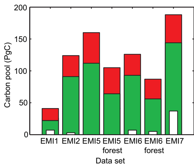
Fig. 3. Comparison of the sum of terrestrial carbon pools (PgC) for the USA in the 1990s. The white color represents the LIT when LIT is separated from SOC. The green color shows the SOC + LIT. The red color denotes the VC.
