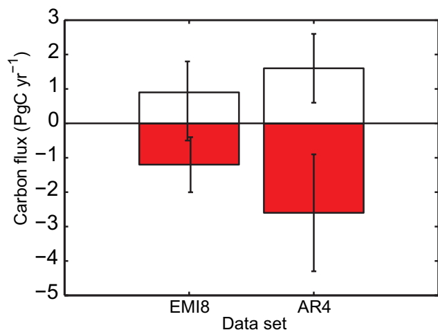
Fig. 2. Comparison of global land-use change fluxes and residual terrestrial sinks ( \text{PgC yr}^{-1} ) in the 1990s. The sign for removal is negative (-) and that for emissions positive (+). The white color represents LUCF. The red color shows ENV.
