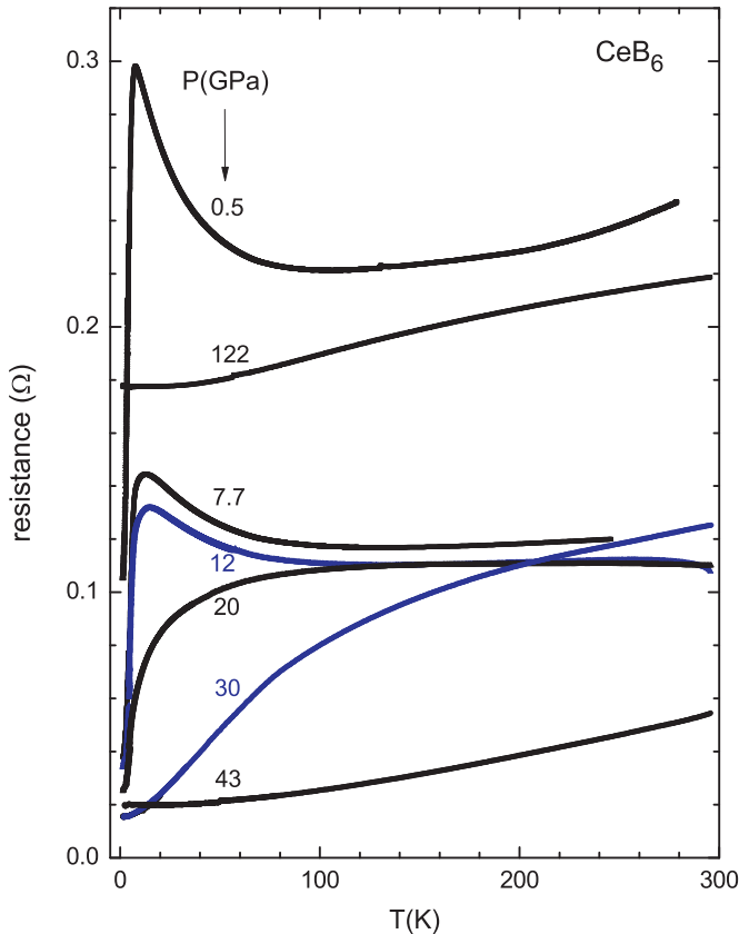
Fig. 2. Electrical resistance of \text{CeB}_6 versus temperature at pressures in GPa measured at 295 K before cooling. Numbers in parentheses after each pressure give pressures measured at 5–10 K after cooling (left) and at 295 K after warming back to 295 K (right): 0.5(1.2, 0.8), 7.7(–0.8.5), 12(–0.14), 20(24.5, –), 30(35, 31), 43 (52, 45), 122(–, 129). A dash “–” indicates the pressure was not measured.
