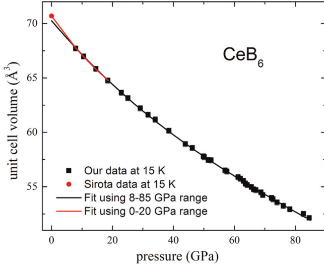
Fig. 4. Pressure dependence of unit cell volume of \text{CeB}_6 at 15 K. Error bars are smaller than symbols. Data are fit 3rd order Birch–Murnaghan equation of state [32]. Black curve fits present data 8–85 GPa. Red curve fits 4 data points 8–20 GPa plus point at 0 GPa from Sirota et al. in Ref. [33]. Fit parameters are given in Table 1. (For interpretation of the references to color in this figure caption, the reader is referred to the web version of this article.)
