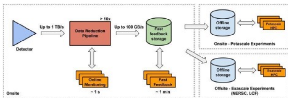
Figure 5.9.1: MEC-U Data System Main Components and Data Flow.
