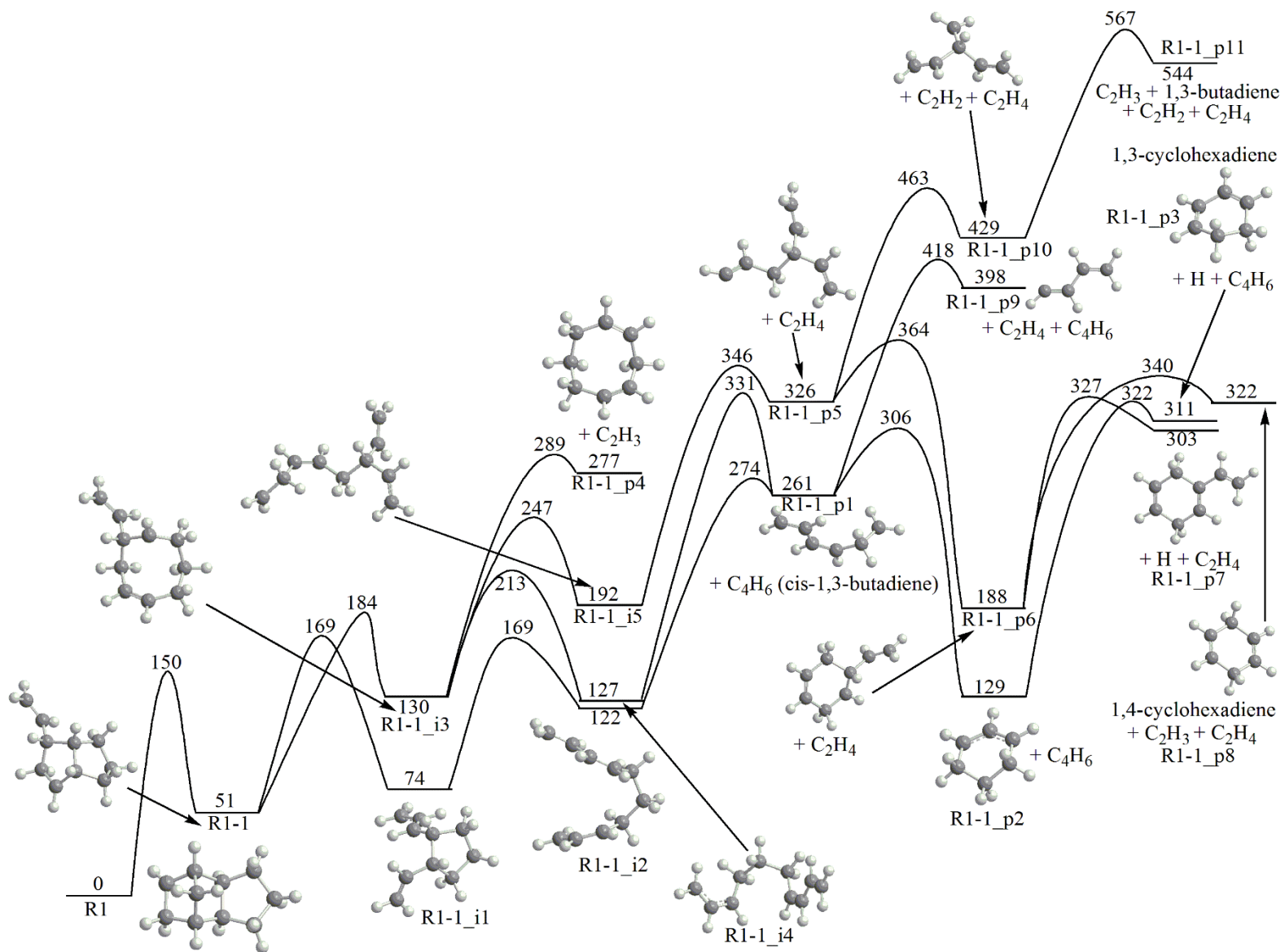
Figure 16. Potential energy diagram for decomposition of R1-1. All relative energies are computed at the G3 level and are given in kJ mol -1 .
