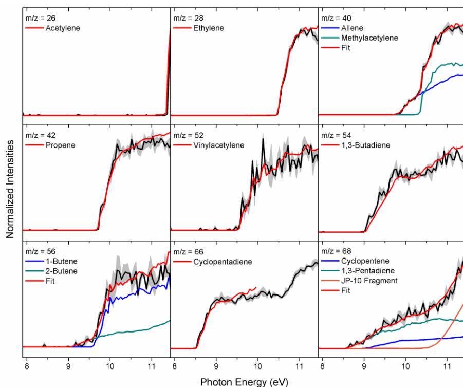
Figure S6-6-1. Experimental photoionization efficiency curves (PIE, black lines) recorded from the decomposition of JP-10 (NSRL) at 1061 K along with the experimental errors (gray area) and the reference PIE curves (blue, green and red lines). In case of multiple contributions to one PIE curve, the red line resembles the overall fit. JP-10 fragment means the photolysis fragment of JP-10. For m/z = 66 and 68 , the PIE curves present sharp increase above 10.5 eV due to photolysis fragment of JP-10.
