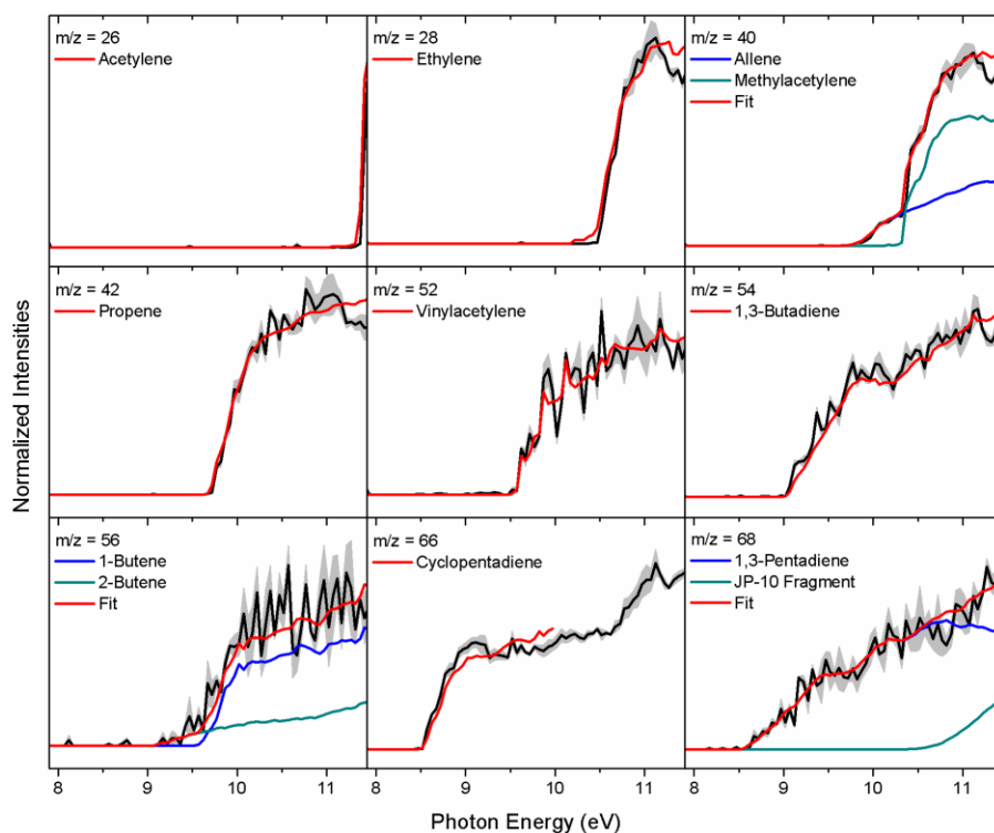
Figure 10-1. Experimental photoionization efficiency curves (PIE, black lines) recorded from the decomposition of JP-10 (NSRL) at 1083 K along with the experimental errors (gray area) and the reference PIE curves (blue, green and red lines). In case of multiple contributions to one PIE curve, the red line resembles the overall fit. JP-10 fragment means the photolysis fragment of JP-10.
