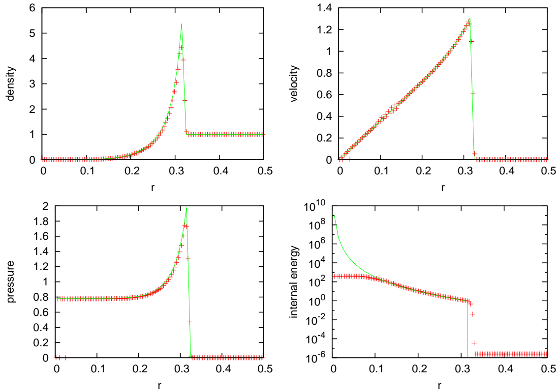
Fig. 8.— CASTRO solution at t = 0.1 s for the cylindrical Sedov blast wave problem run in 2D Cartesian coordinates. This was run with a base grid with \Delta x = 0.03125 cm and 3 levels of factor 2 refinement for an effective resolution of \Delta x = .00390625 cm.
