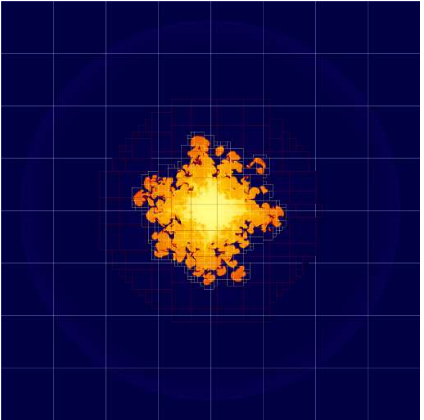
Fig. 15.— Here we see a 2D slice of the temperature field from a 3D calculation of a Type Ia supernova with two levels of refinement. There are 512 grids, each containing 64^3 cells, at the coarsest level, over 1000 grids at level 1 and over 2000 grids at level 2. Approximately 1.8% of the domain is at the finest resolution.
