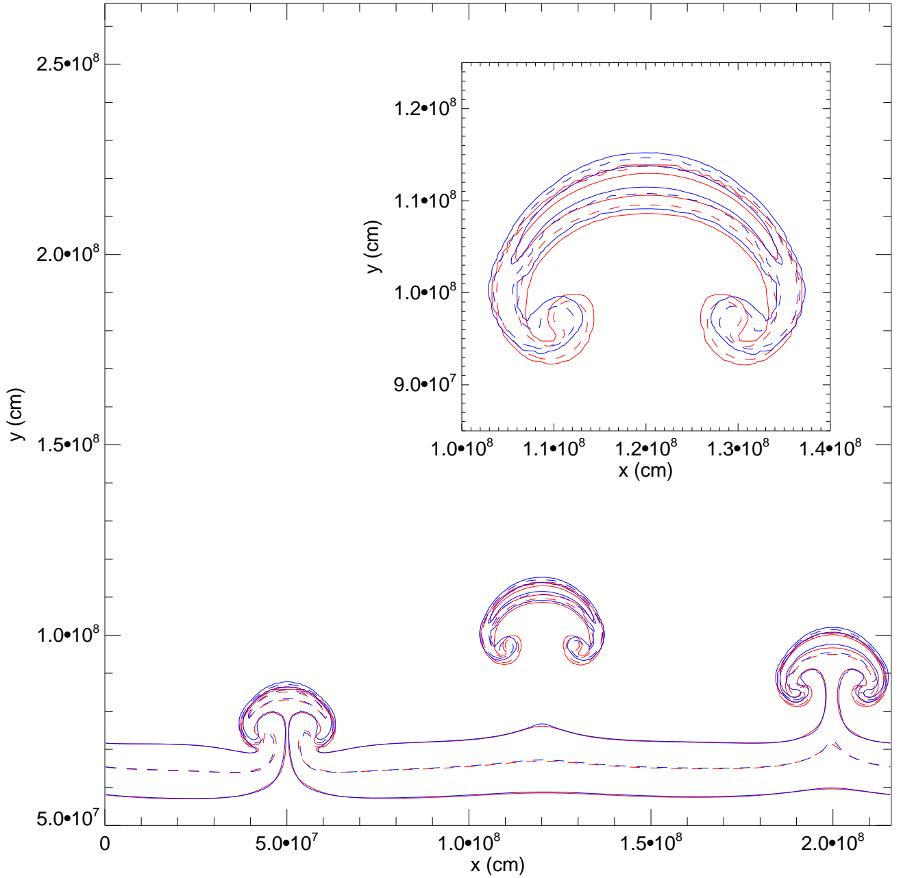
Fig. 14.— Comparison of FLASH (red) and CASTRO (blue) ^{24}\text{Mg} mass fraction contours for the reacting bubble test. Contours are drawn at values of X of 5 \times 10^{-9} , 5 \times 10^{-8} , 5 \times 10^{-7} , 5 \times 10^{-6} , with alternating solid and dashed lines. The inset shows the detail of the middle bubble. As with the temperature, we see good agreement between FLASH and CASTRO.
