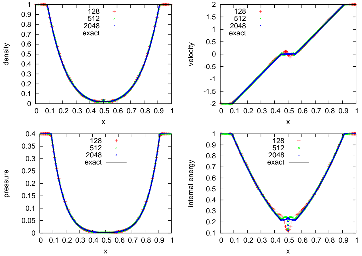
Fig. 4.— Adaptive CASTRO solutions vs. analytic solution for the double rarefaction problem run in 1D at effective resolutions of 128, 512 and 2048 cells.
