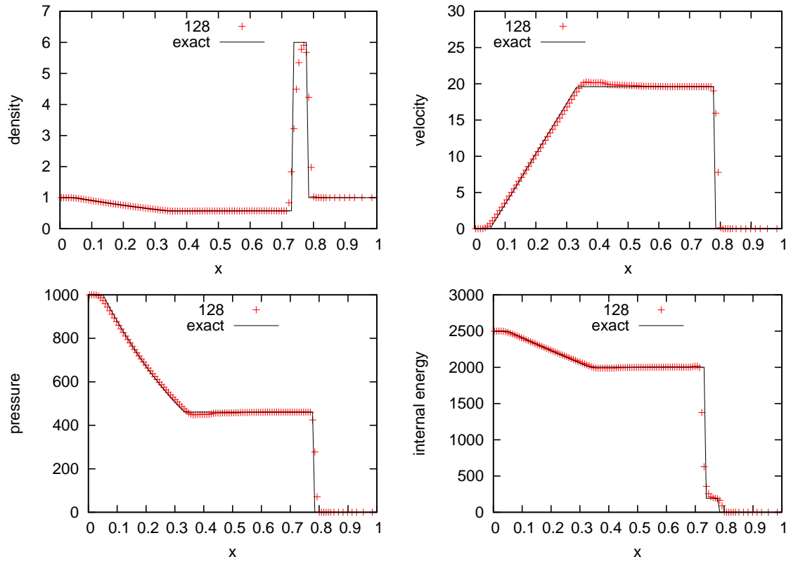
Fig. 5.— Adaptive CASTRO solution vs. analytic solution for the strong shock problem run in 1D at an effective resolution of 128 cells.
