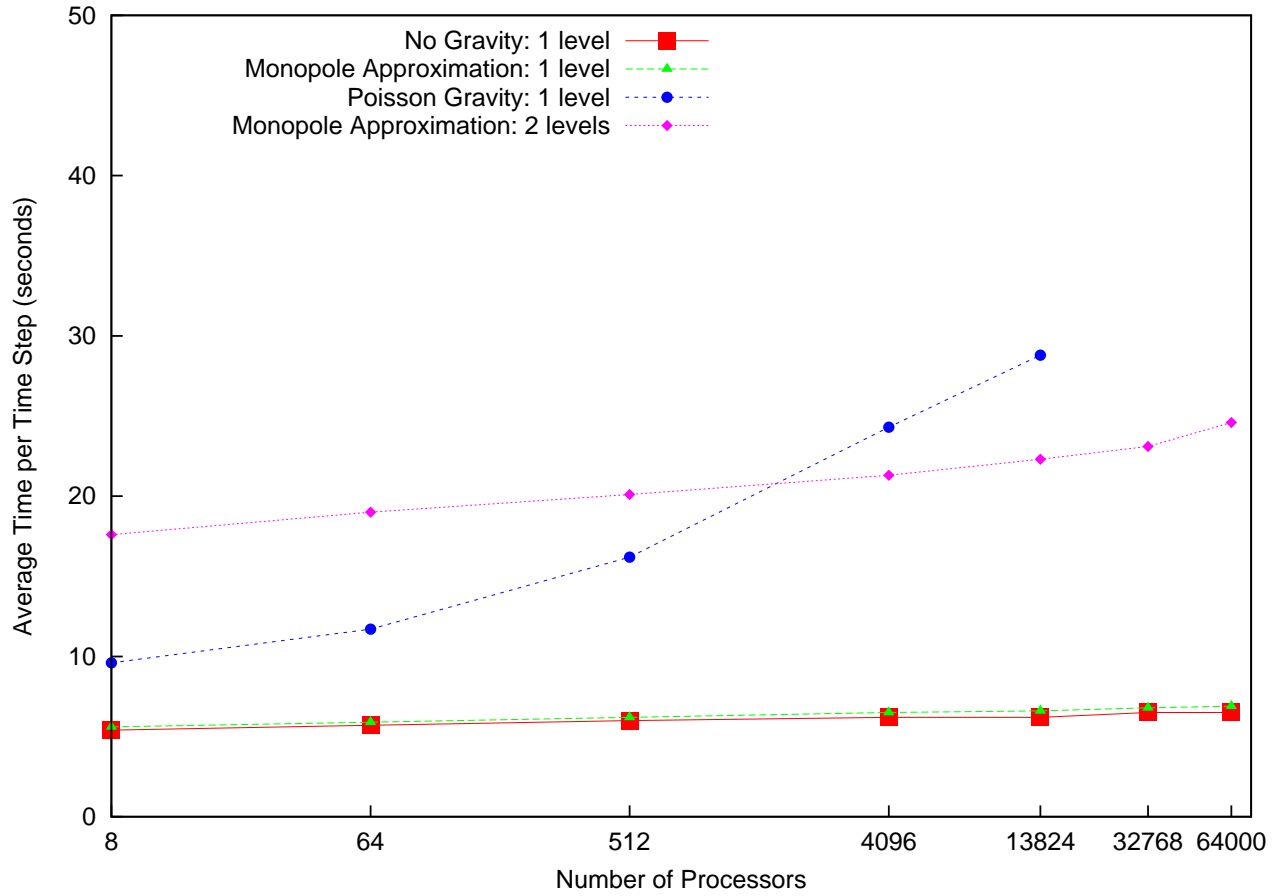
Fig. 2.— Weak scaling behavior of the CASTRO code on the jaguarpf machine at the OLCF. For the two-level simulation, the number of cells that are advanced in a time step increases by a factor of three because of subcycling. To quantify the overall performance, we note that for the 64,000 processor case without gravity, the time for a single core to advance one cell for one time step is 24.8 \mu\text{s} .
