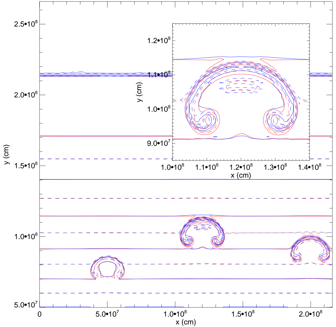
Fig. 13.— Comparison of FLASH (red) and CASTRO (blue) temperature contours for the reacting bubble test. Temperature contours at 10^8 , 1.5 \times 10^8 , 2 \times 10^8 , 2.5 \times 10^8 , 3. \times 10^8 , 3.5 \times 10^8 , 4. \times 10^8 , 4.5 \times 10^8 , 5. \times 10^8 , 5.5 \times 10^8 , 6. \times 10^8 , 6.5 \times 10^8 , 7. \times 10^8 , 7.5 \times 10^8 , 8. \times 10^8 K are shown, drawn with alternating solid and dashed lines. The inset shows the detail of the middle bubble. We see good agreement between FLASH and CASTRO.
