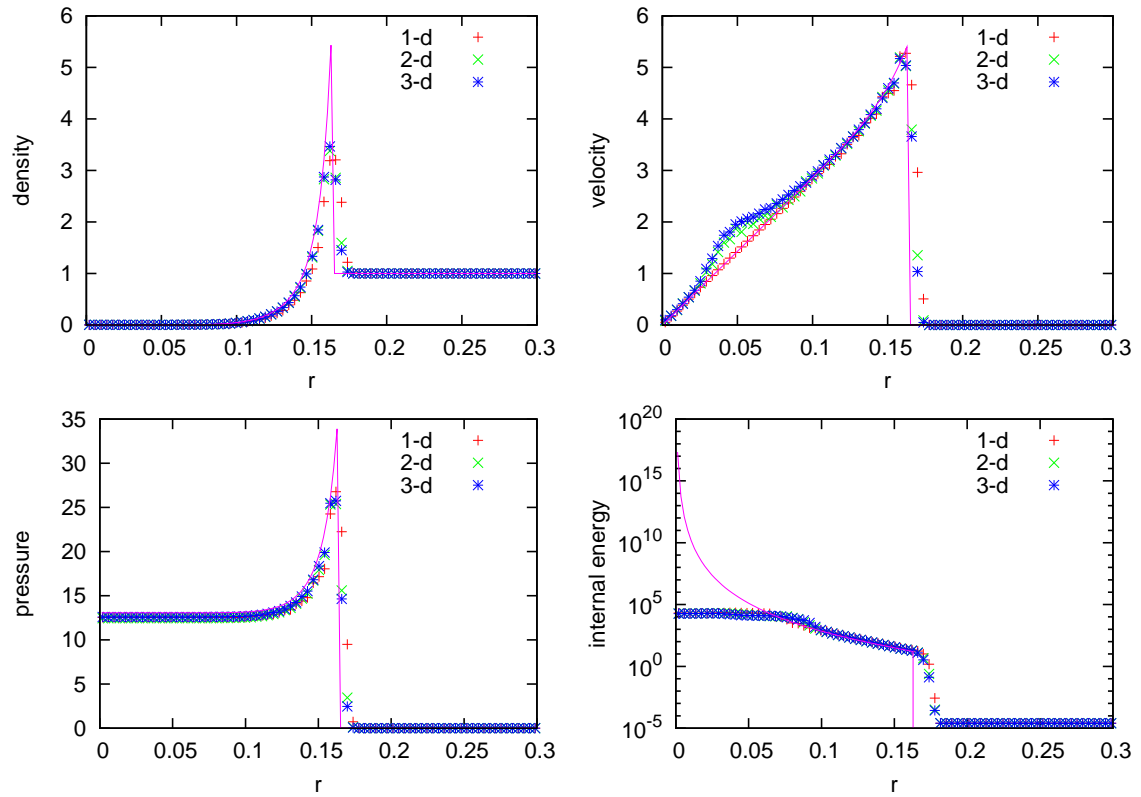
Fig. 6.— CASTRO solution at t = 0.01 s for the spherical Sedov blast wave problem run in 1D spherical, 2D axisymmetric, and 3D Cartesian coordinates. This was run with a base grid with \Delta x = 0.03125 cm and 3 levels of factor 2 refinement for an effective resolution of \Delta x = .00390625 cm.
