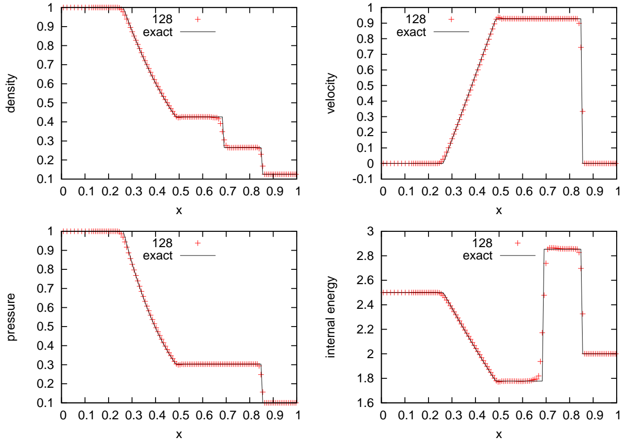
Fig. 3.— Adaptive CASTRO solution vs. analytic solution for Sod’s problem run in 1D at an effective resolution of 128 cells.
