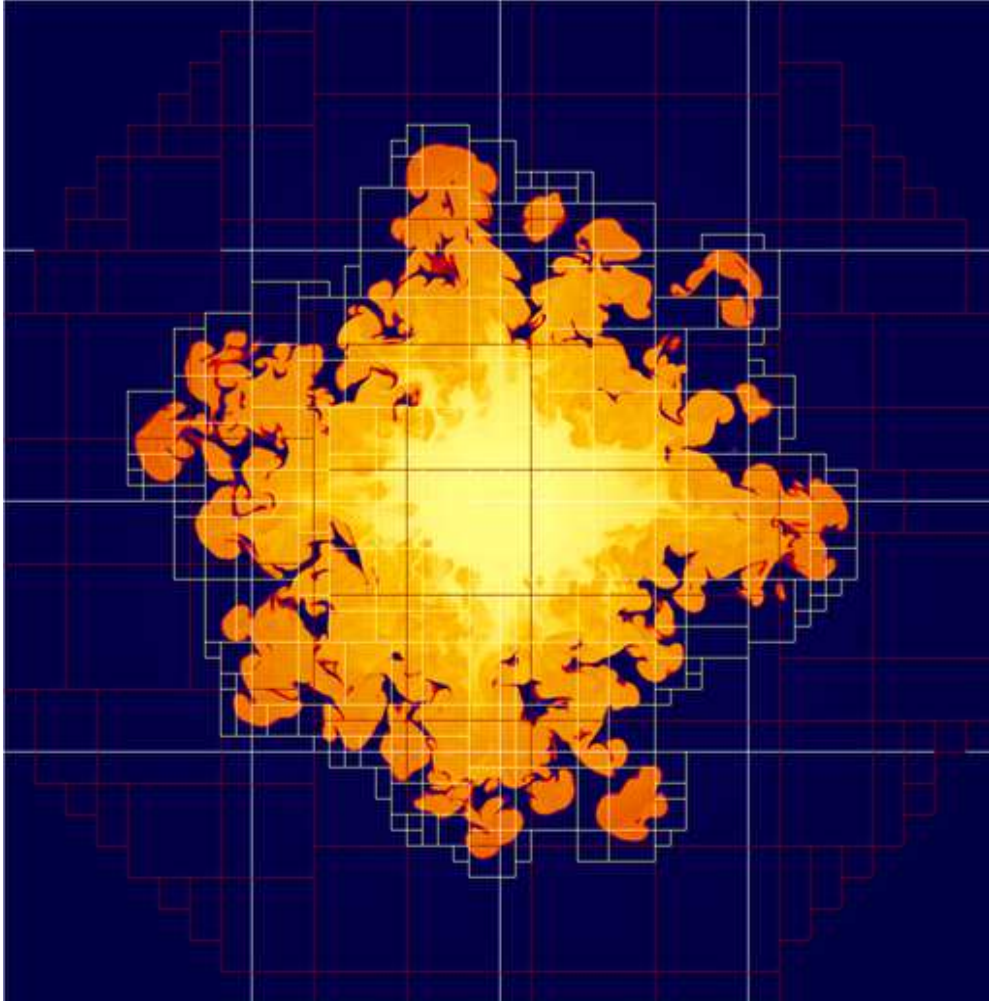
Fig. 16.— Here we see a close-up of the previous figure, showing more detail of the level 2 grids.
