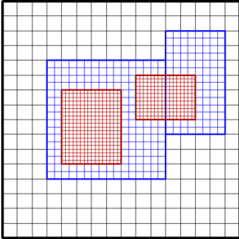
Fig. 1.— Cartoon of AMR grids with two levels of factor 2 refinement. The black grid covers the domain with 16^2 cells. Bold lines represent grid boundaries, the different colors represent different levels of refinement. The two blue grids are at level 1 and the cells are a factor of two finer than those at level 0. The two red grids are at level 2 and the cells are a factor of two finer than the level 1 cells. Note that the level 2 grids are properly nested within the union of level 1 grids, but there is no direct parent-child connection.
