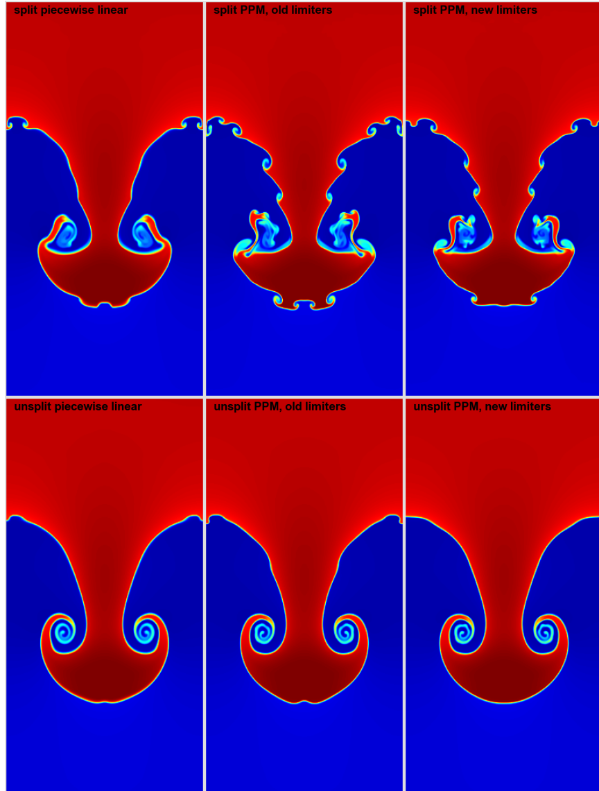
Fig. 9.— Density in a single-mode Rayleigh-Taylor simulation for a variety of advection schemes. Dimensionally-split method results are shown on the top row; unsplit method results are shown on the bottom row. We see that the unsplit methods do better at suppressing the growth of high-wavenumber instabilities resulting from grid effects.
