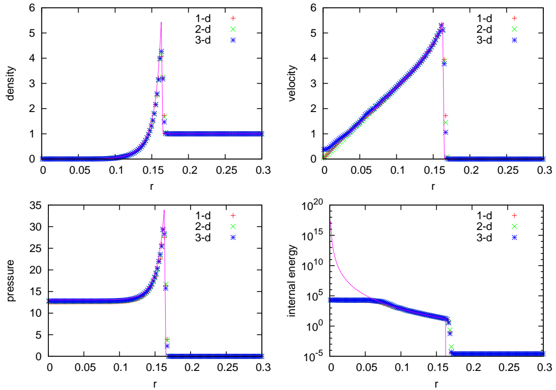
Fig. 7.— CASTRO solution at t = 0.01 s for the spherical Sedov blast wave problem run in 1D spherical, 2D axisymmetric, and 3D Cartesian coordinates. This was run with a base grid with \Delta x = 0.03125 cm and 4 levels of factor 2 refinement for an effective resolution of \Delta x = .001953125 cm.
