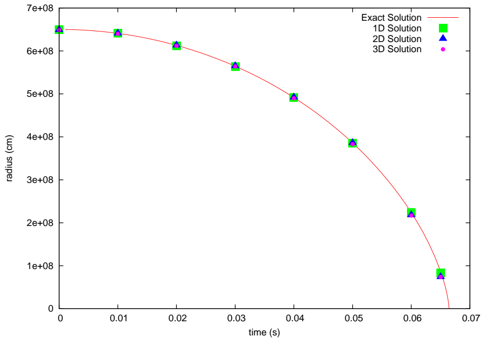
Fig. 12.— Radius vs. time for the homologous dust collapse problem in 1D, 2D, and 3D simulations as compared to the exact solution. In all three cases we see excellent agreement with the exact solution.
