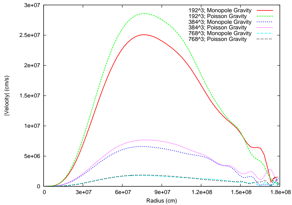
Fig. 11.— Magnitude of velocity vs. radius at t = 1 s for the stationary star gravity problem. At each of the three resolutions, we show the results using a monopole gravity approximation and Poisson solve for gravity. Here, we see clear second order convergence in the max norm, and the monopole and Poisson simulations agree best at the highest resolution.
