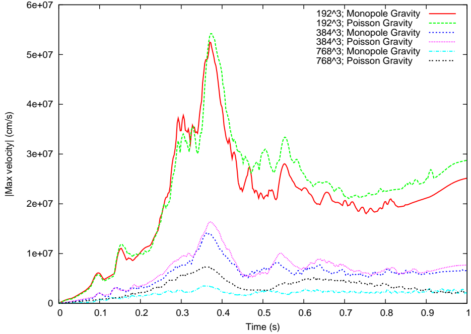
Fig. 10.— Maximum magnitude of velocity vs. time for the stationary star gravity problem. At each of the three resolutions, we show the results using a monopole gravity approximation and Poisson solve for gravity. We note that in each simulation, the maximum velocity is not strictly increasing, leading us to believe that over longer periods of time the velocities will remain small. We note that sound speed at the center of the star is approximately 9.4 \times 10^8 cm/s, so at the highest resolution, the peak velocity is less than 1% of the sound speed. The solutions in the monopole and Poisson cases match up very well; the discrepancy we see at the finest resolution is due to large velocities at the edge of the star, which is typically outside the region of interest.
